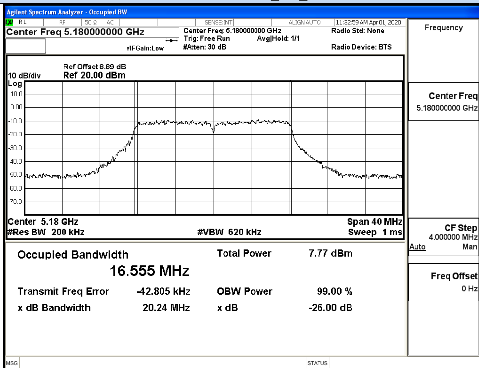
26dB Bandwidth_Ant_0
