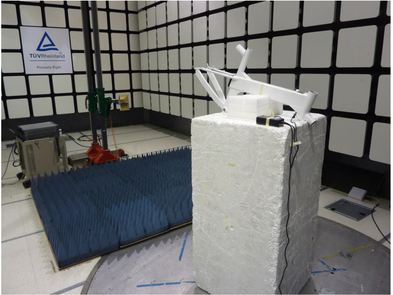
Figure 3: Test Setup for 1 GHz to 18 GHz
