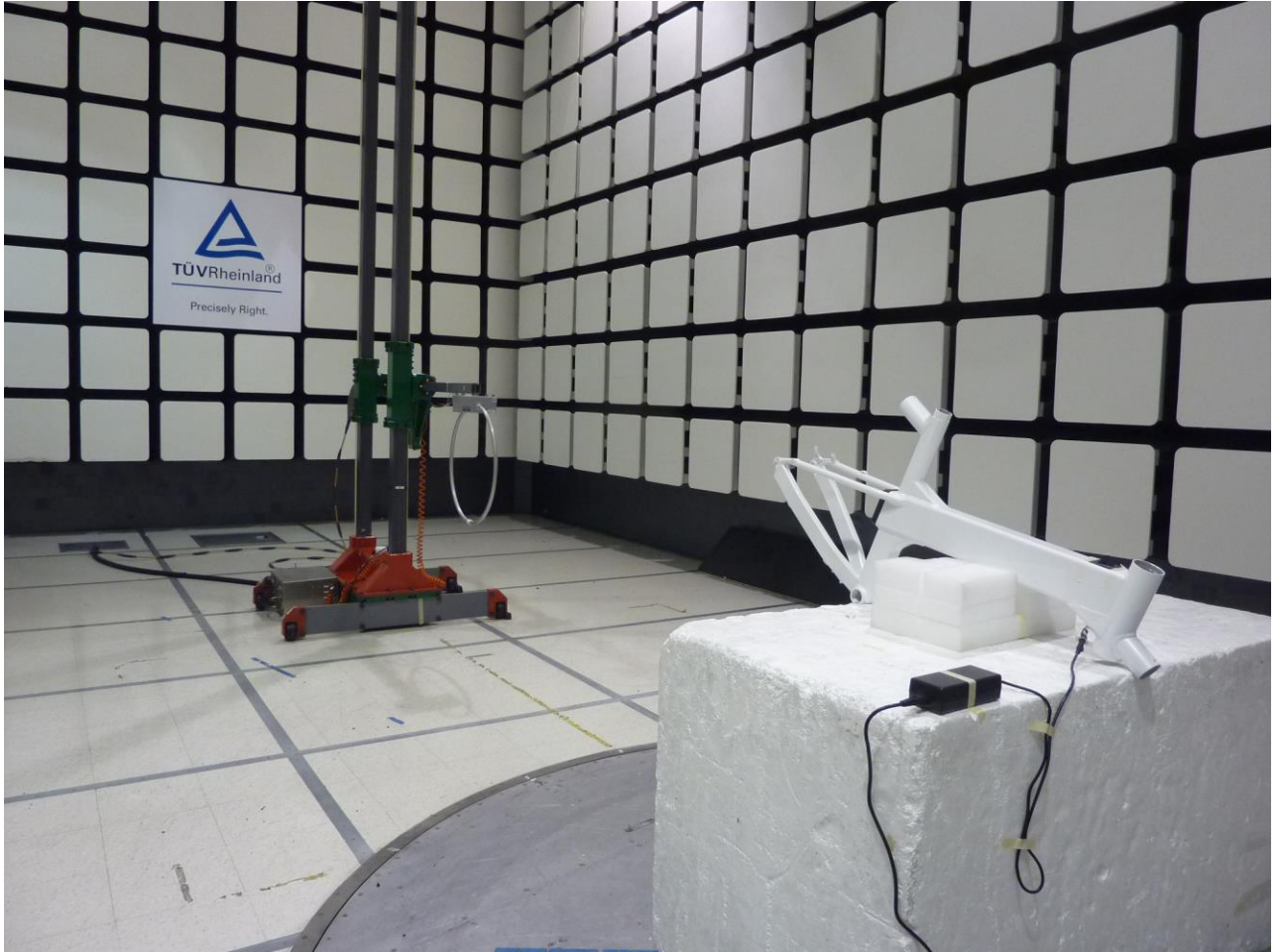
Figure 1: Test Setup for 9 kHz to 30 MHz
