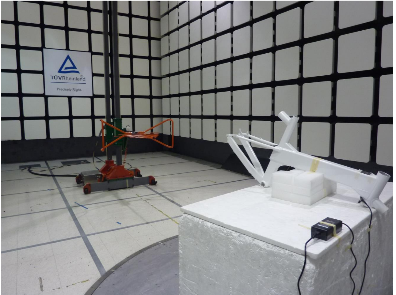
Figure 2: Test Setup for 30 MHz to 1000 MHz
