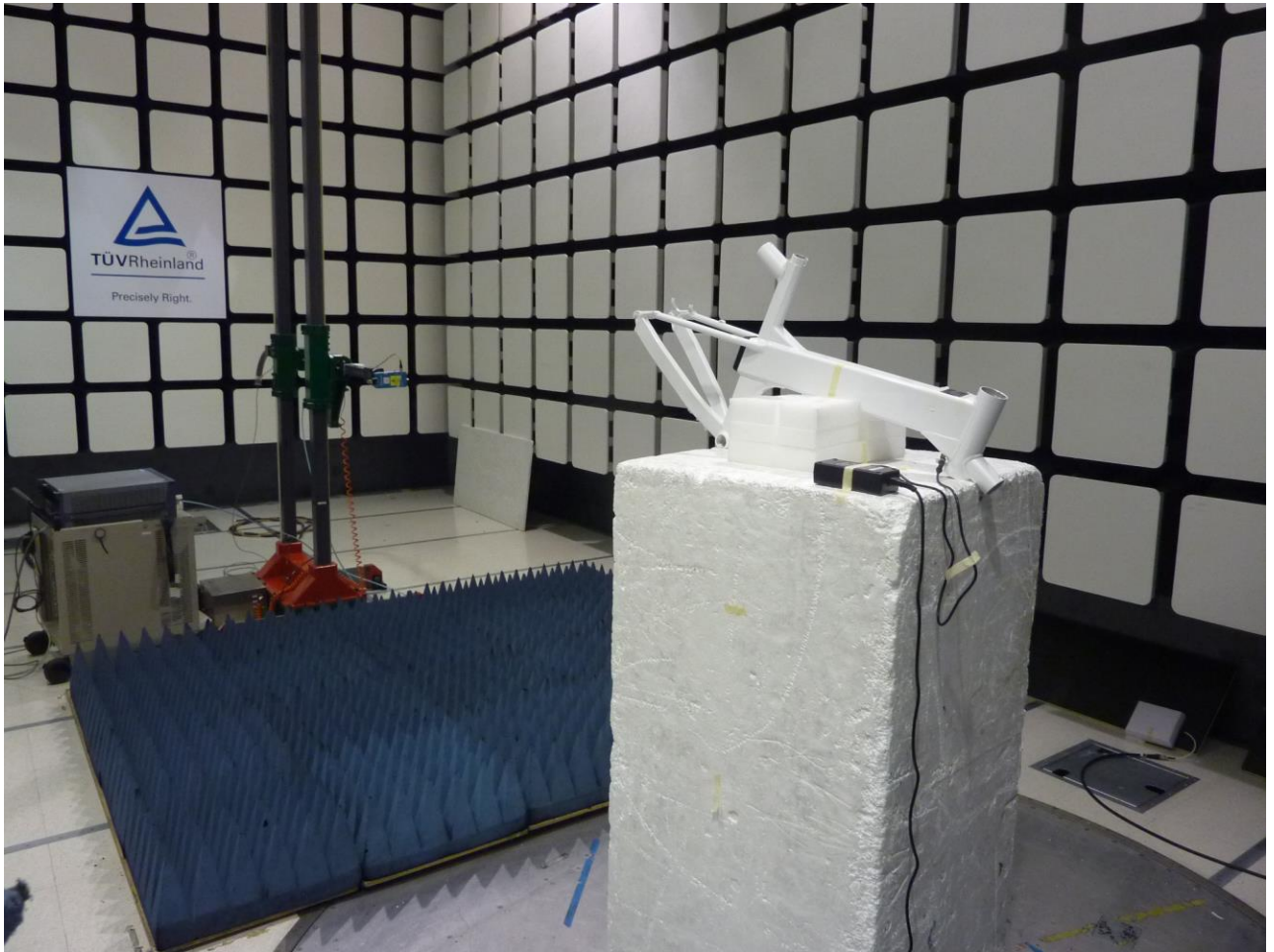
Figure 4: Test Setup for 18 GHz to 26 GHz
