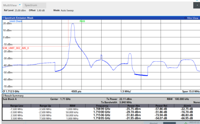
Band66-5MHz-QPSK-132647-1RB#24
