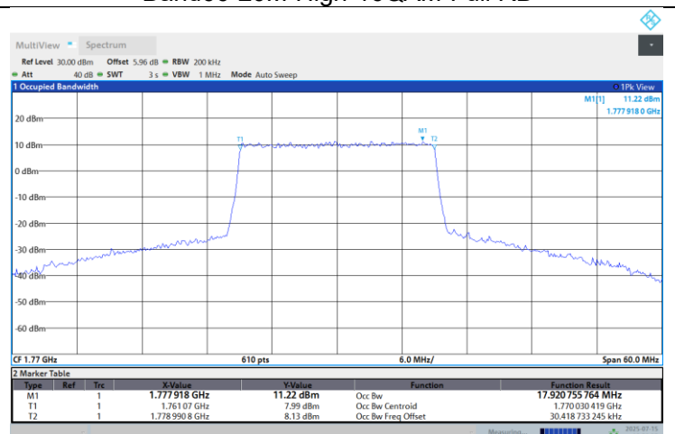
Band66-20M-High-16QAM-Full RB
