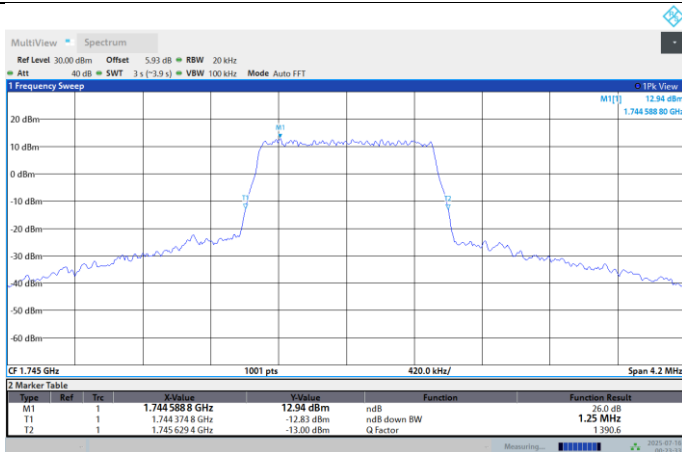
Band66-1.4M-Mid-QPSK-Full RB
