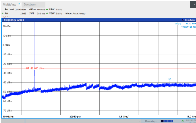
Band41-5MHz-QPSK-40620-1RB#0- Range:30~15000MHz
