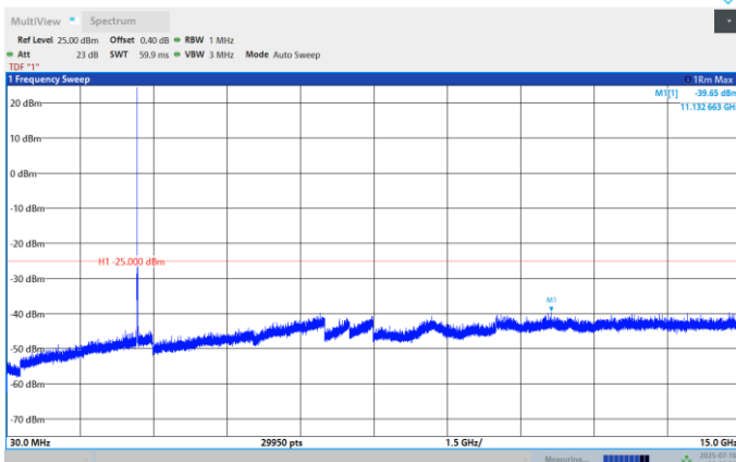
Band41-10MHz-QPSK-39700-1RB#0- Range:30~15000MHz
