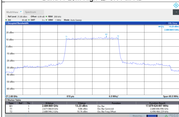
Band41-20M-High-QPSK-Full RB
