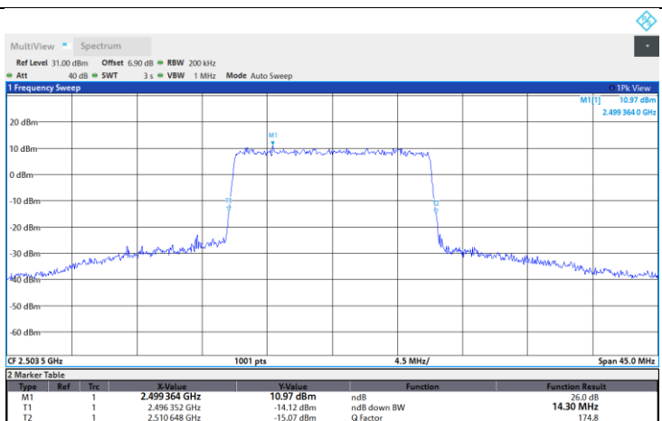
Band41-15M-Mid-16QAM-Full RB
