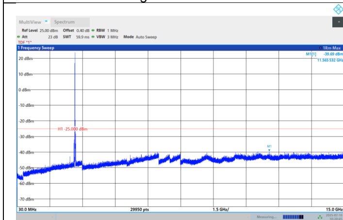
Band41-20MHz-QPSK-41490-1RB#0- Range:30~15000MHz
