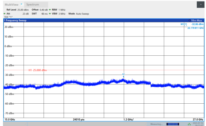
Band41-5MHz-QPSK-40620-1RB#0- Range:15000~27000MHz
