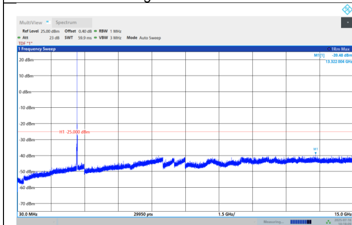
Band41-20MHz-QPSK-39750-1RB#0- Range:30~15000MHz
