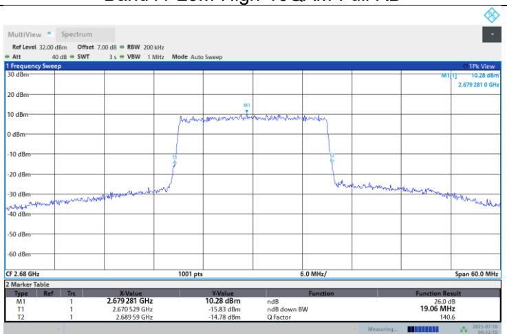
Band41-20M-High-16QAM-Full RB
