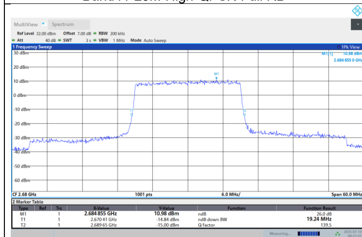
Band41-20M-High-QPSK-Full RB
