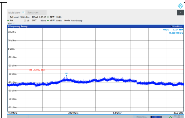
Band41-10MHz-QPSK-40620-1RB#0- Range:15000~27000MHz
