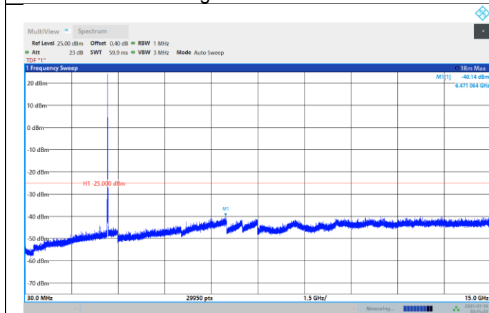
Band41-15MHz-QPSK-39725-1RB#0- Range:30~15000MHz
