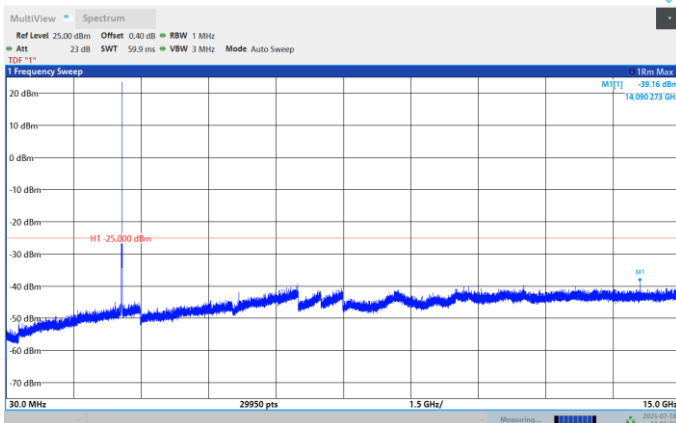
Band41-5MHz-QPSK-41565-1RB#0- Range:30~15000MHz
