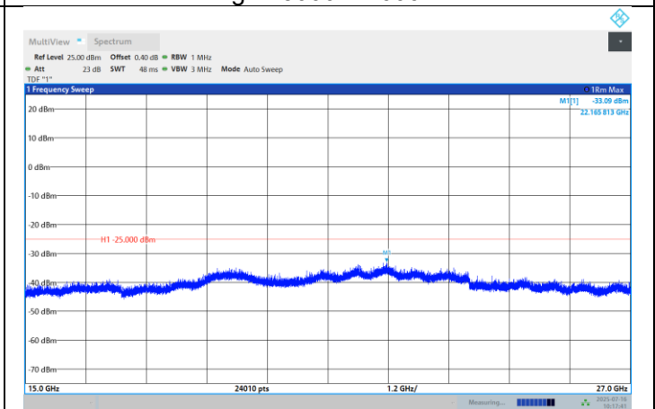
Band41-15MHz-QPSK-41515-1RB#0- Range:15000~27000MHz
