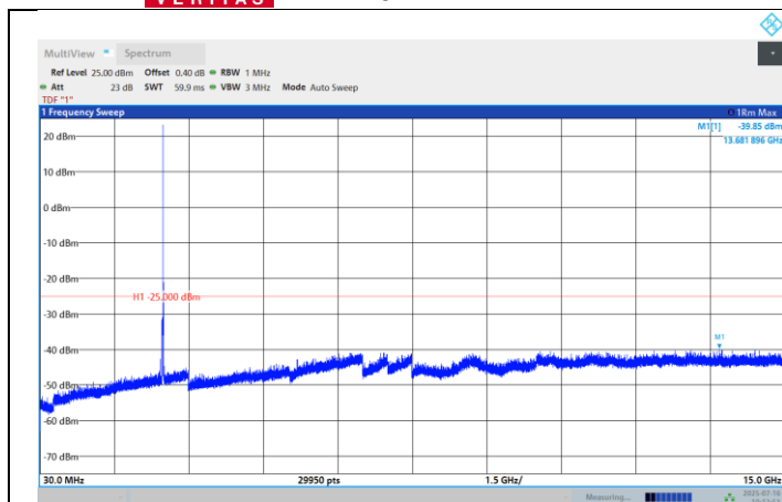
Band41-10MHz-QPSK-40620-1RB#0- Range:30~15000MHz
