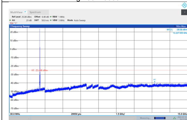
Band41-15MHz-QPSK-41515-1RB#0- Range:30~15000MHz
