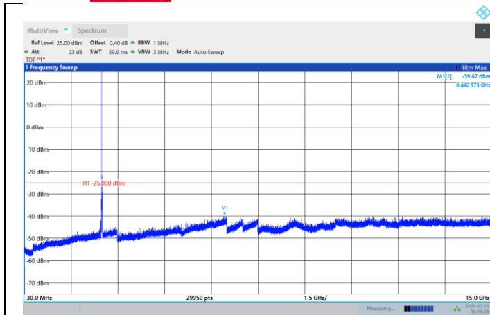
Band41-15MHz-QPSK-40620-1RB#0- Range:30~15000MHz
