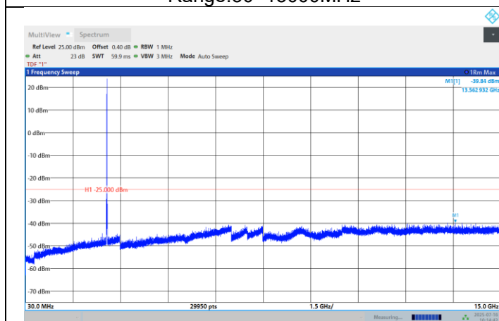
Band41-10MHz-QPSK-41540-1RB#0- Range:30~15000MHz
