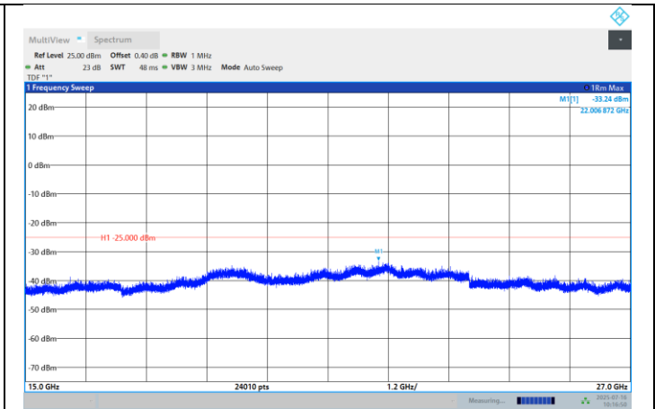
Band41-15MHz-QPSK-40620-1RB#0- Range:15000~27000MHz
