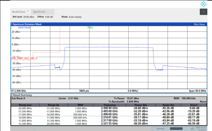
Band41-20MHz-16QAM-41490-100RB#0
