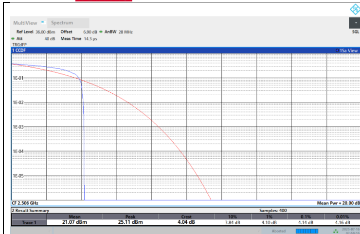
Band41-20M-Low-16QAM-1RB Low
