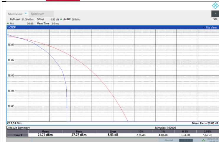
Band41-20M-Low-16QAM-1RB Low
