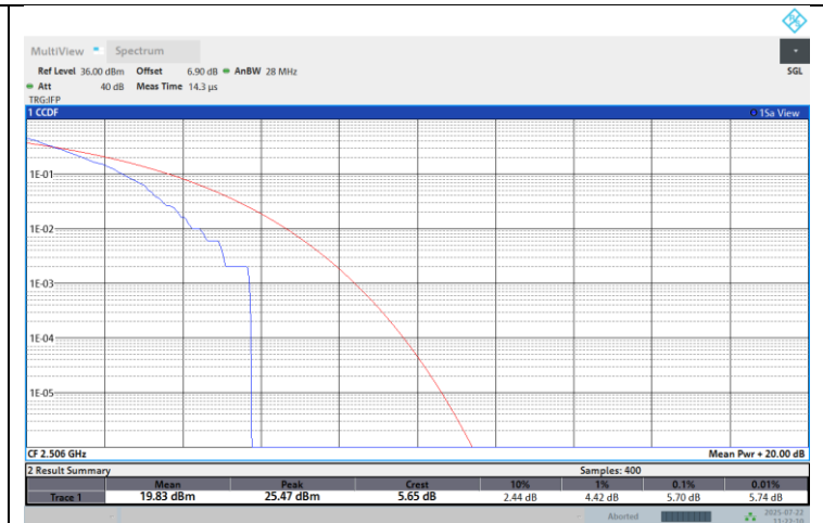
Band41-20M-Low-16QAM-Full RB
