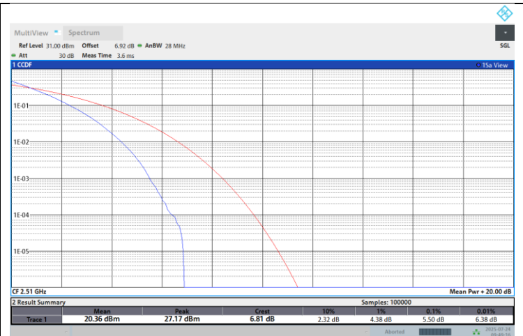
Band41-20M-Low-16QAM-Full RB
