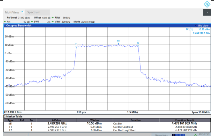
Band41-5M-Mid-16QAM-Full RB
