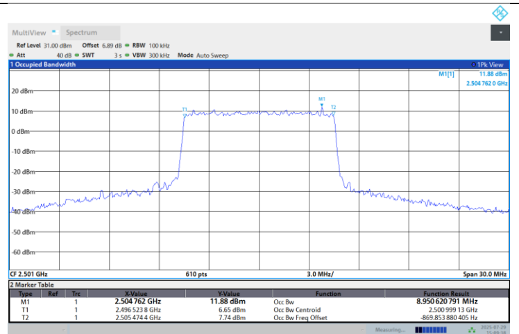
Band41-10M-Mid-16QAM-Full RB
