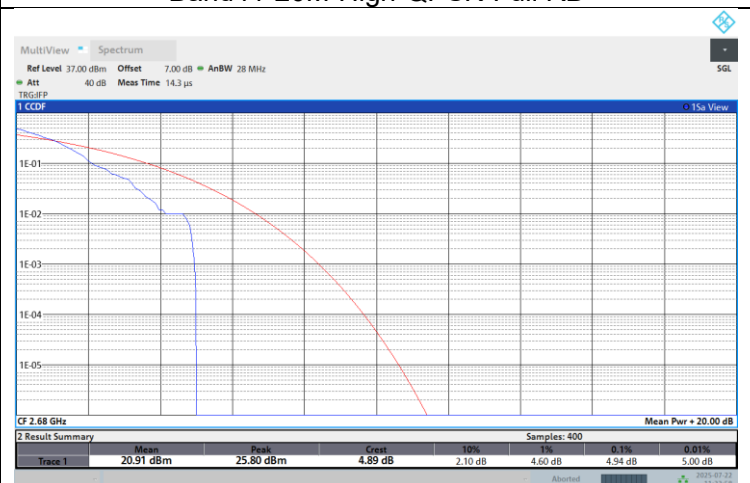
Band41-20M-High-16QAM-Full RB
