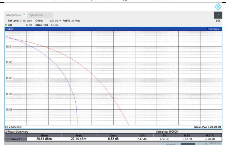
Band41-20M-Mid-16QAM-Full RB
