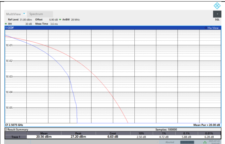
Band41-15M-Low-16QAM-Full RB
