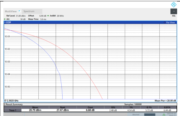
Band41-5M-Low-16QAM-Full RB
