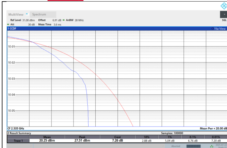
Band41-20M-High-QPSK-1RB Low
