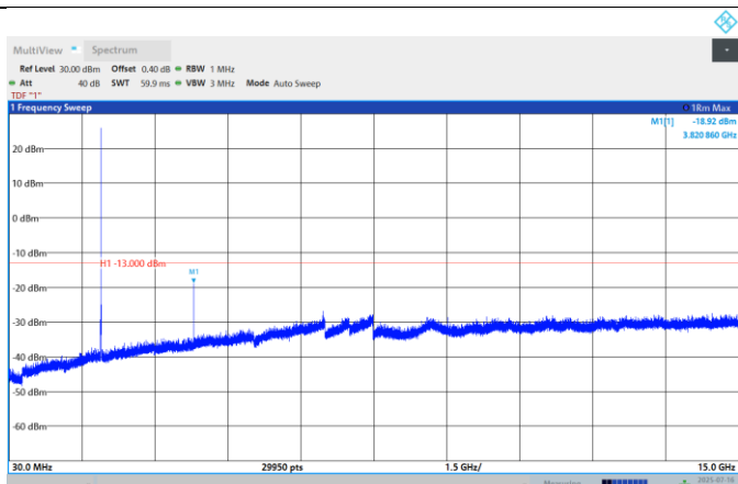
Band25-10MHz-QPSK-26090-1RB#0-Range:30~15000MHz
