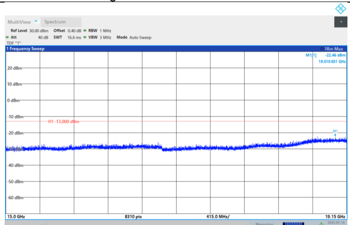
Band25-3MHz-QPSK-26675-1RB#0- Range:15000MHz~19150MHz
