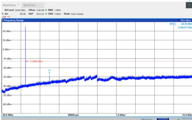
Band25-1.4MHz-QPSK-26683-1RB#0- Range:30~15000MHz
