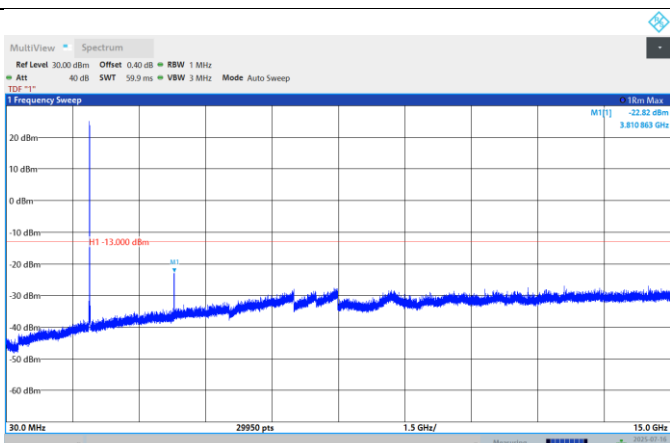
Band25-15MHz-QPSK-26115-1RB#0-Range:30~15000MHz
