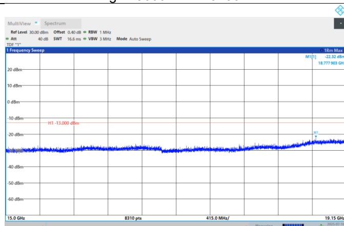
Band25-10MHz-QPSK-26090-1RB#0- Range:15000MHz~19150MHz
