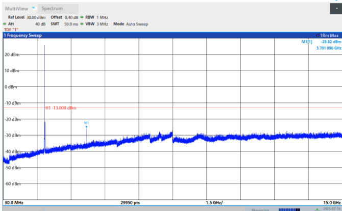
Band25-15MHz-QPSK-26340-1RB#0-Range:30~15000MHz
