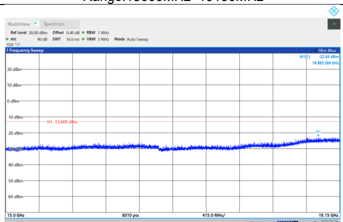
Band25-5MHz-QPSK-26065-1RB#0- Range:15000MHz~19150MHz
