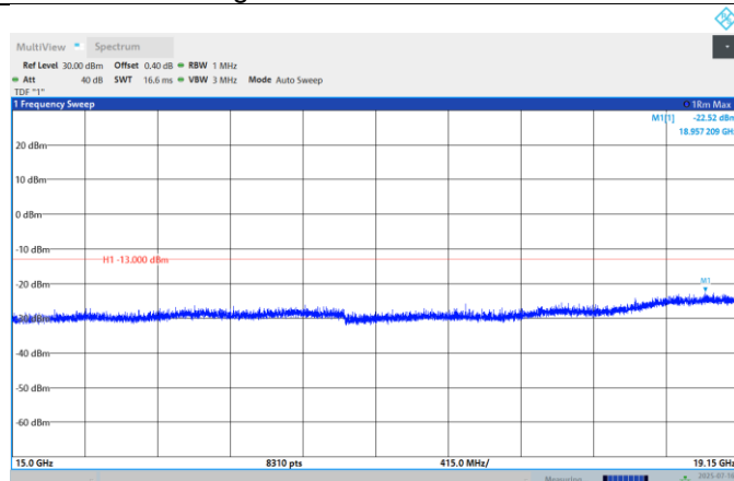
Band25-5MHz-QPSK-26665-1RB#0- Range:15000MHz~19150MHz
