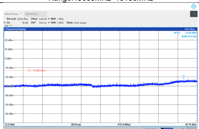
Band25-15MHz-QPSK-26115-1RB#0- Range:15000MHz~19150MHz
