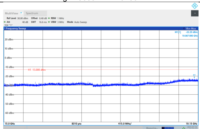
Band25-20MHz-QPSK-26140-1RB#0- Range:15000MHz~19150MHz
