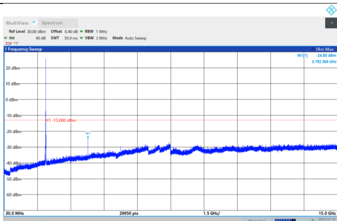
Band25-20MHz-QPSK-26590-1RB#0-Range:30~15000MHz
