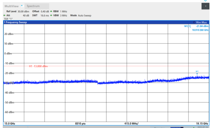
Band25-3MHz-QPSK-26055-1RB#0- Range:15000MHz~19150MHz
