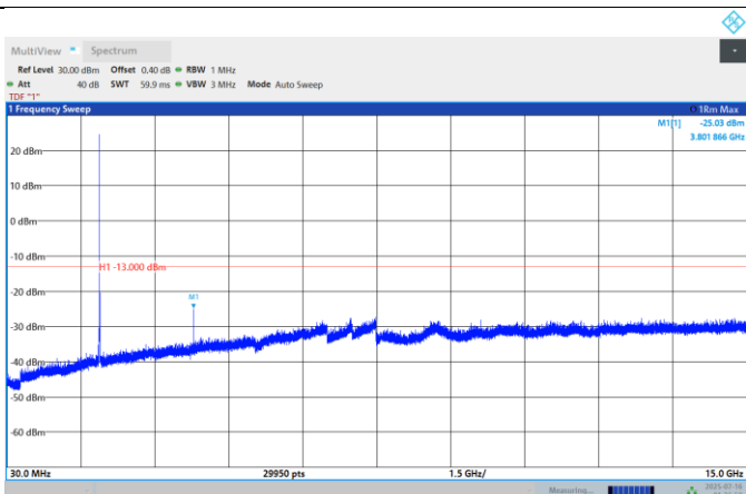
Band25-20MHz-QPSK-26140-1RB#0-Range:30~15000MHz
