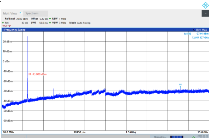
Band25-10MHz-QPSK-26640-1RB#0-Range:30~15000MHz
