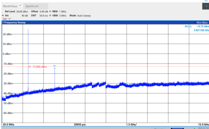
Band25-3MHz-QPSK-26055-1RB#0-Range:30~15000MHz
