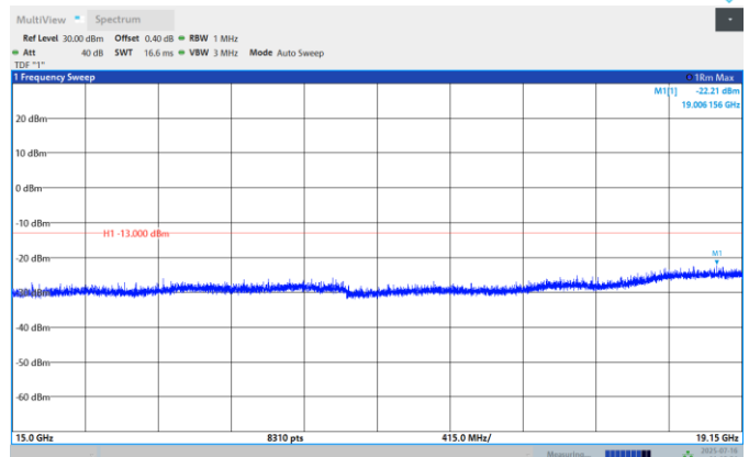
Band25-1.4MHz-QPSK-26683-1RB#0- Range:15000MHz~19150MHz
