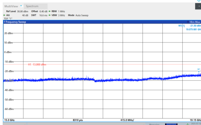
Band25-5MHz-QPSK-26340-1RB#0- Range:15000MHz~19150MHz
