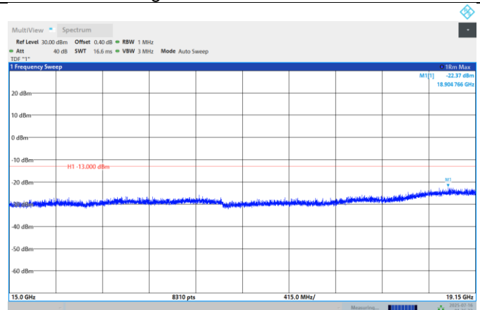
Band25-15MHz-QPSK-26615-1RB#0- Range:15000MHz~19150MHz
