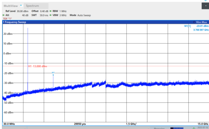
Band25-3MHz-QPSK-26340-1RB#0-Range:30~15000MHz
