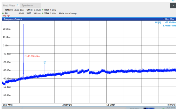
Band25-5MHz-QPSK-26340-1RB#0-Range:30~15000MHz
