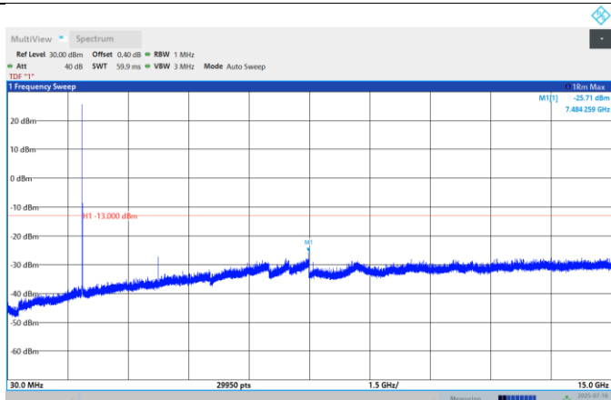
Band25-5MHz-QPSK-26665-1RB#0-Range:30~15000MHz
