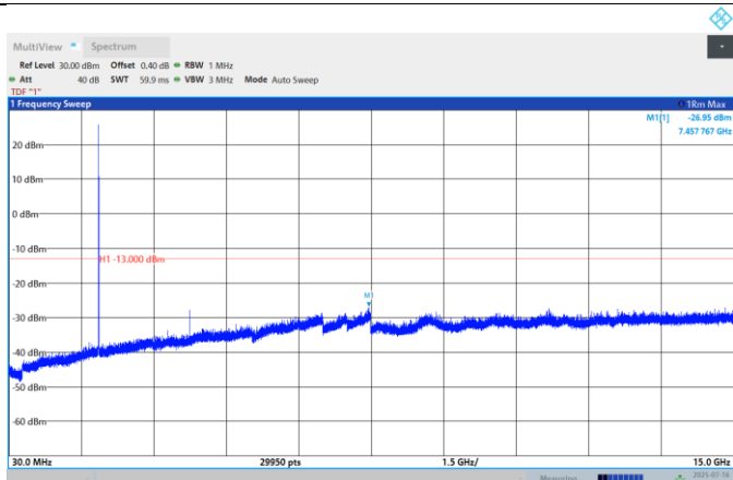
Band25-3MHz-QPSK-26675-1RB#0-Range:30~15000MHz
