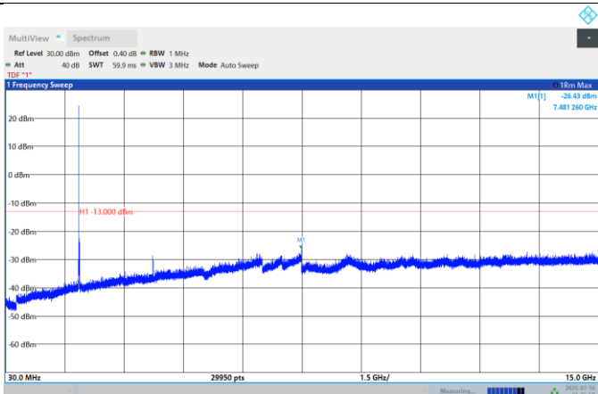
Band25-15MHz-QPSK-26615-1RB#0-Range:30~15000MHz
