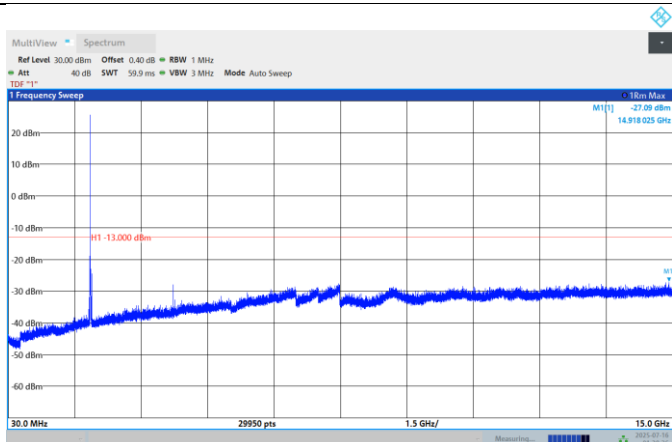
Band25-20MHz-QPSK-26590-1RB#0-Range:30~15000MHz
