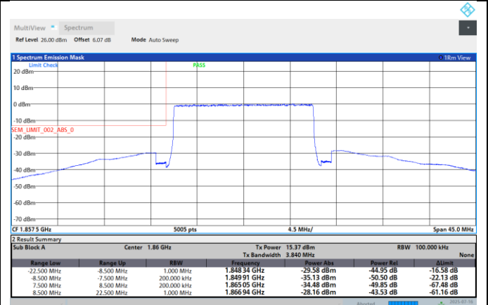
Band25-15MHz-QPSK-26615-75RB#0
