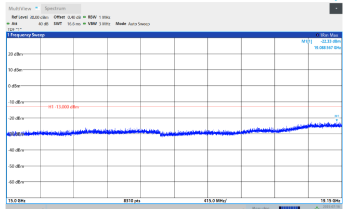
Band25-15MHz-QPSK-26340-1RB#0- Range:15000MHz~19150MHz
