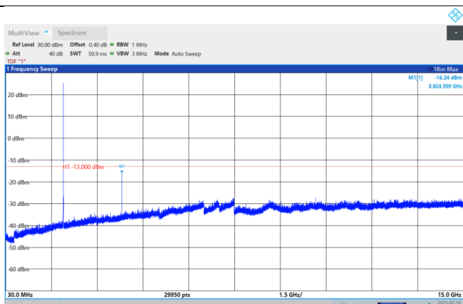
Band25-5MHz-QPSK-26065-1RB#0-Range:30~15000MHz
