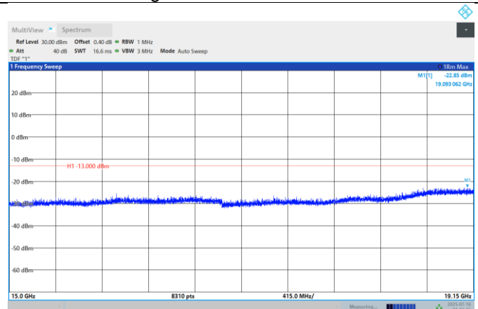
Band25-10MHz-QPSK-26640-1RB#0- Range:15000MHz~19150MHz
