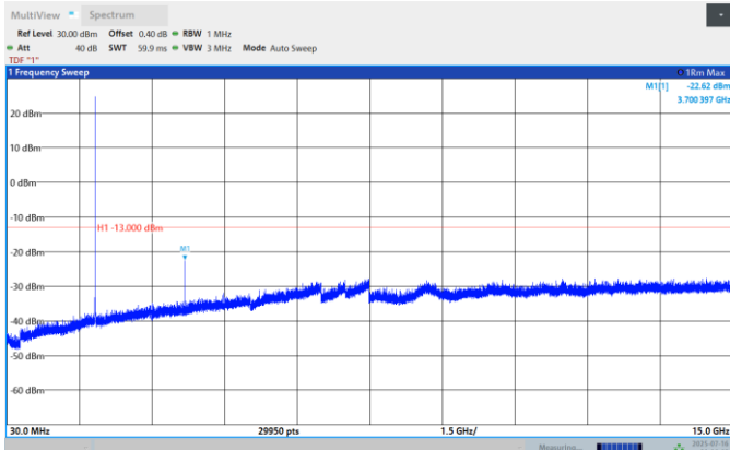
Band25-1.4MHz-QPSK-26340-1RB#0- Range:30~15000MHz
