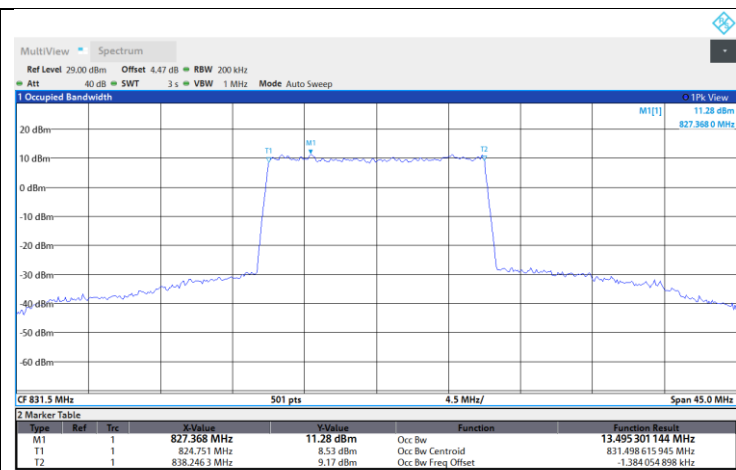
Band26-15M-Mid-16QAM-Full RB
