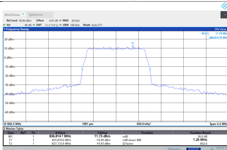
Band26-1.4M-High-16QAM-Full RB
