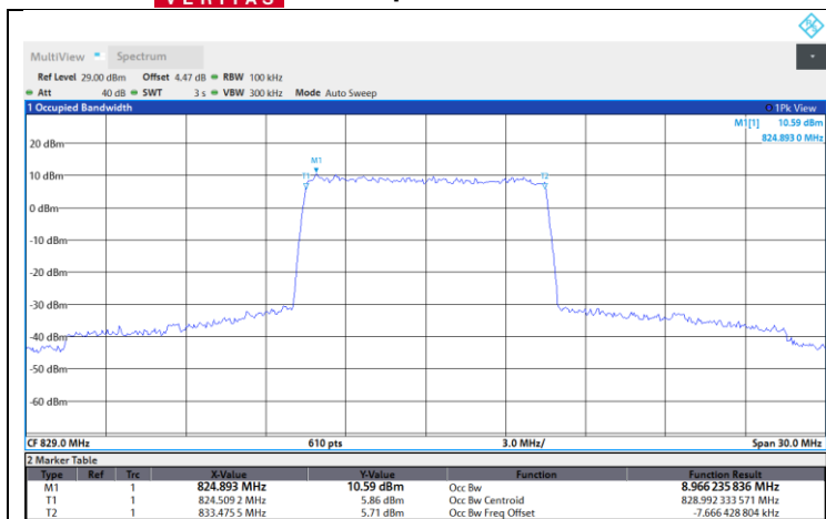
Band26-10M-Mid-QPSK-Full RB
