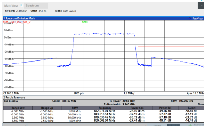
Band26-5MHz-16QAM-26815-25RB#0
