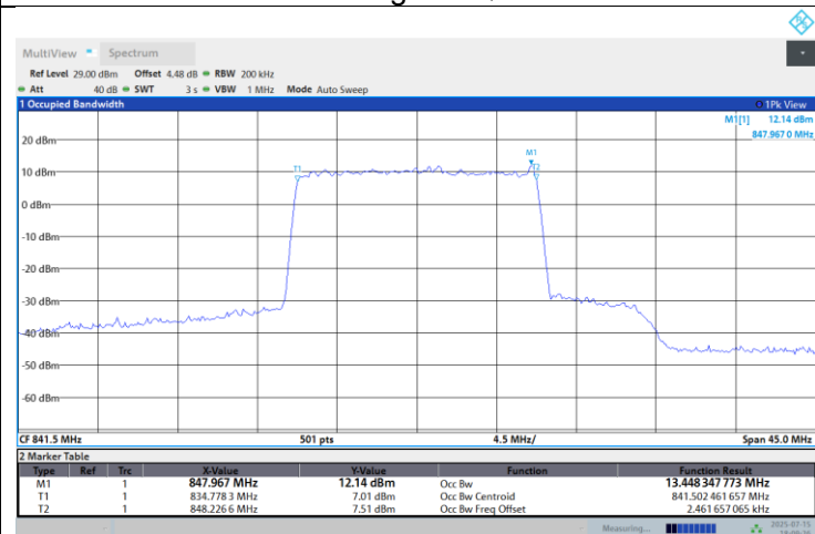
Band26-15M-High-16QAM-Full RB
