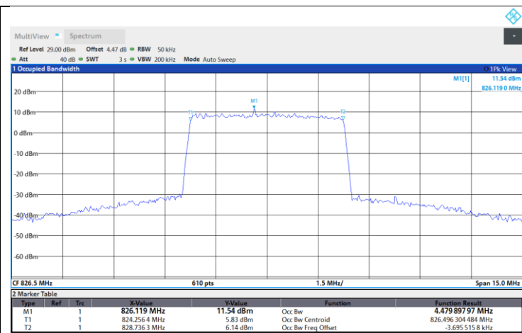
Band26-5M-Mid-16QAM-Full RB
