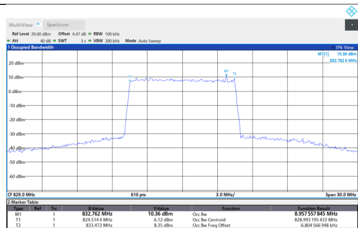
Band26-10M-Mid-16QAM-Full RB
