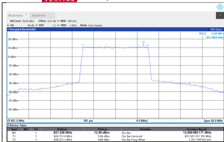
Band26-15M-Mid-QPSK-Full RB
