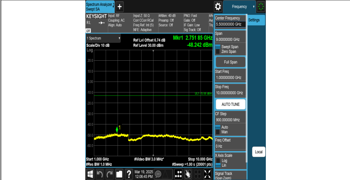
Band26(814-824)-5MHz-16QAM-26740-1RB#24-30-1000-PASS
