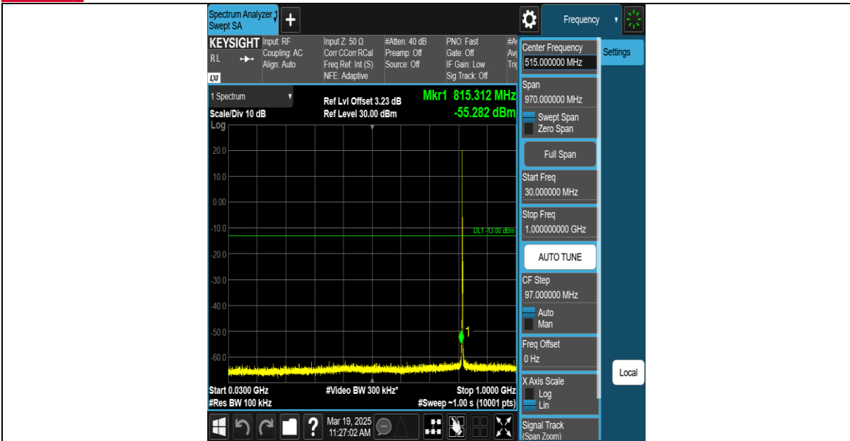
Band26(814-824)-1.4MHz-QPSK-26740-1RB#0-1000~1000-PASS
