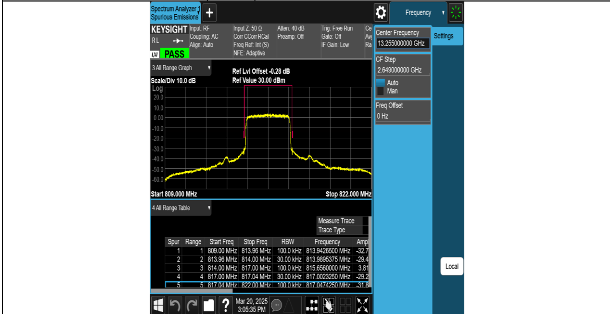
Band26(814-824)-3MHz-QPSK-26775-15RB#0-PASS
