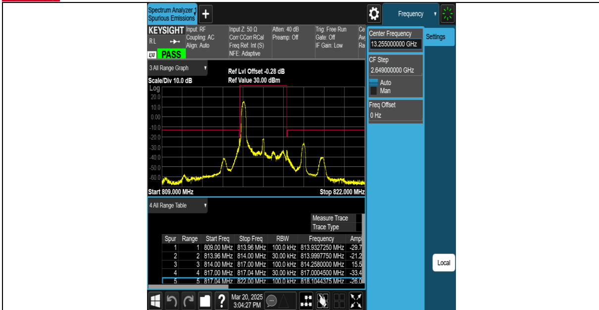
Band26(814-824)-3MHz-QPSK-26705-15RB#0-PASS
