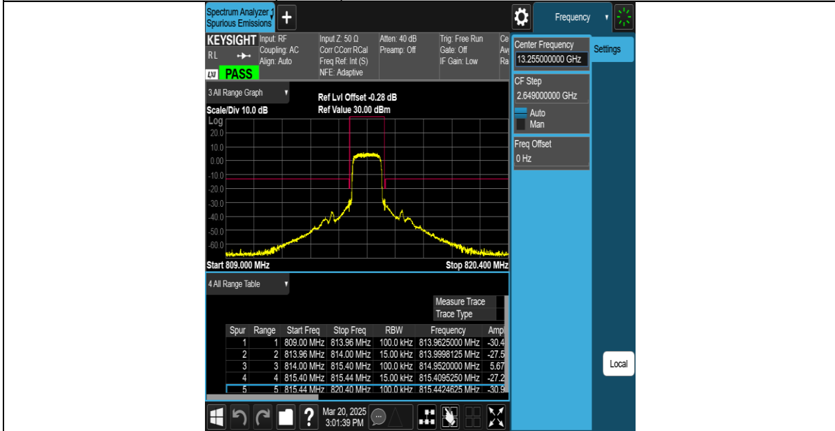
Band26(814-824)-1.4MHz-16QAM-26783-6RB#0-PASS
