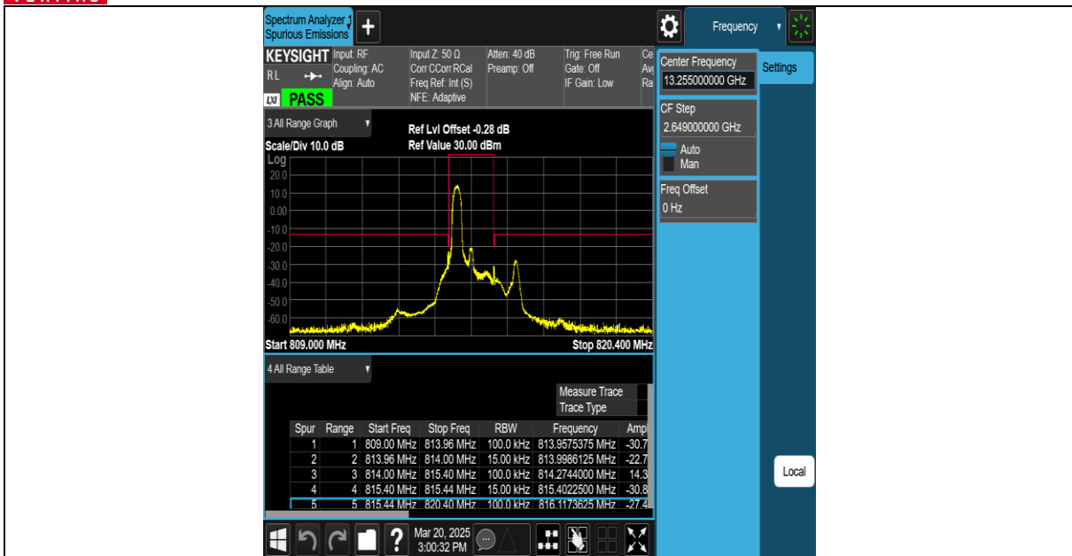
Band26(814-824)-1.4MHz-16QAM-26697-6RB#0-PASS
