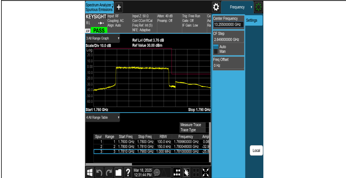
Band66-15MHz-QPSK-132597-1RB#74-PASS
