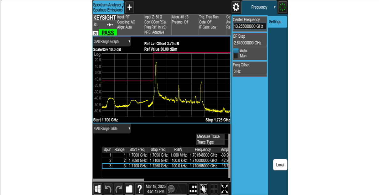
Band66-10MHz-16QAM-132022-27RB#0-PASS
