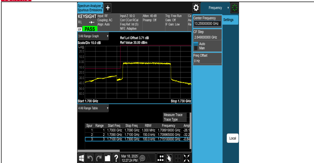
Band66-15MHz-QPSK-132597-75RB#0-PASS
