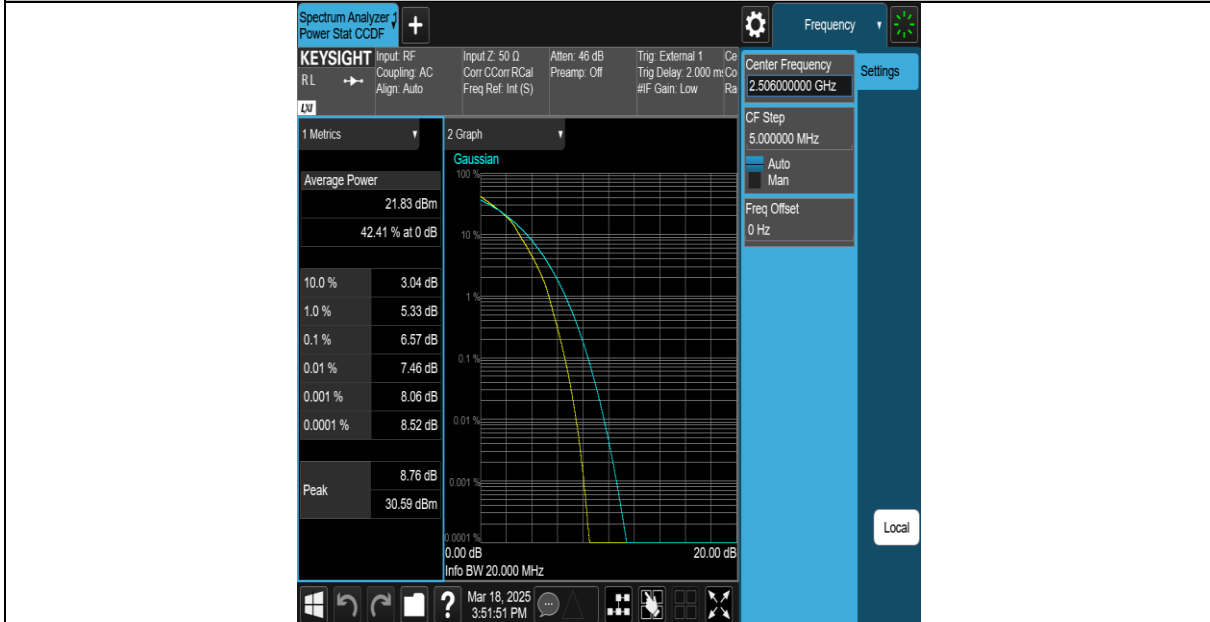
Band41-20MHz-16QAM-40620-1RB#0-PASS
