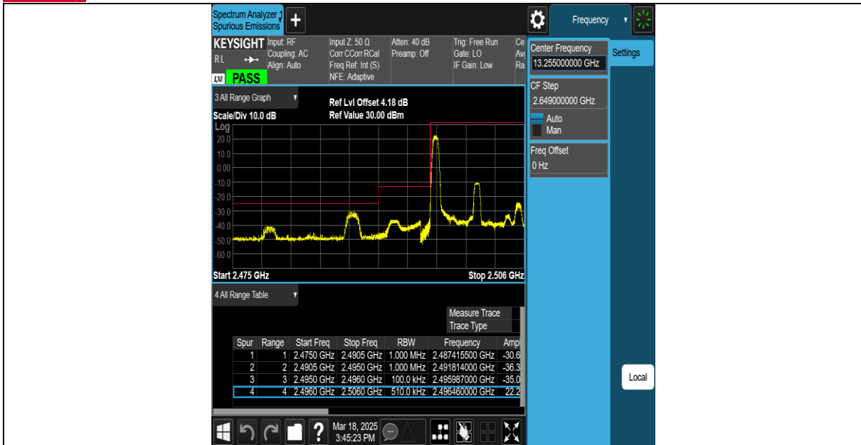
Band41-10MHz-16QAM-39700-27RB#0-PASS
