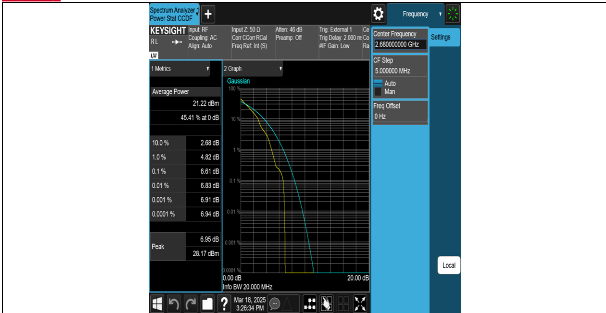
Band41-20MHz-QPSK-41490-100RB#0-PASS
