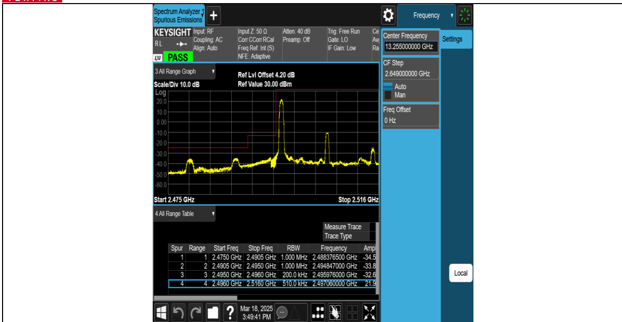
Band41-20MHz-16QAM-39750-27RB#0-PASS
