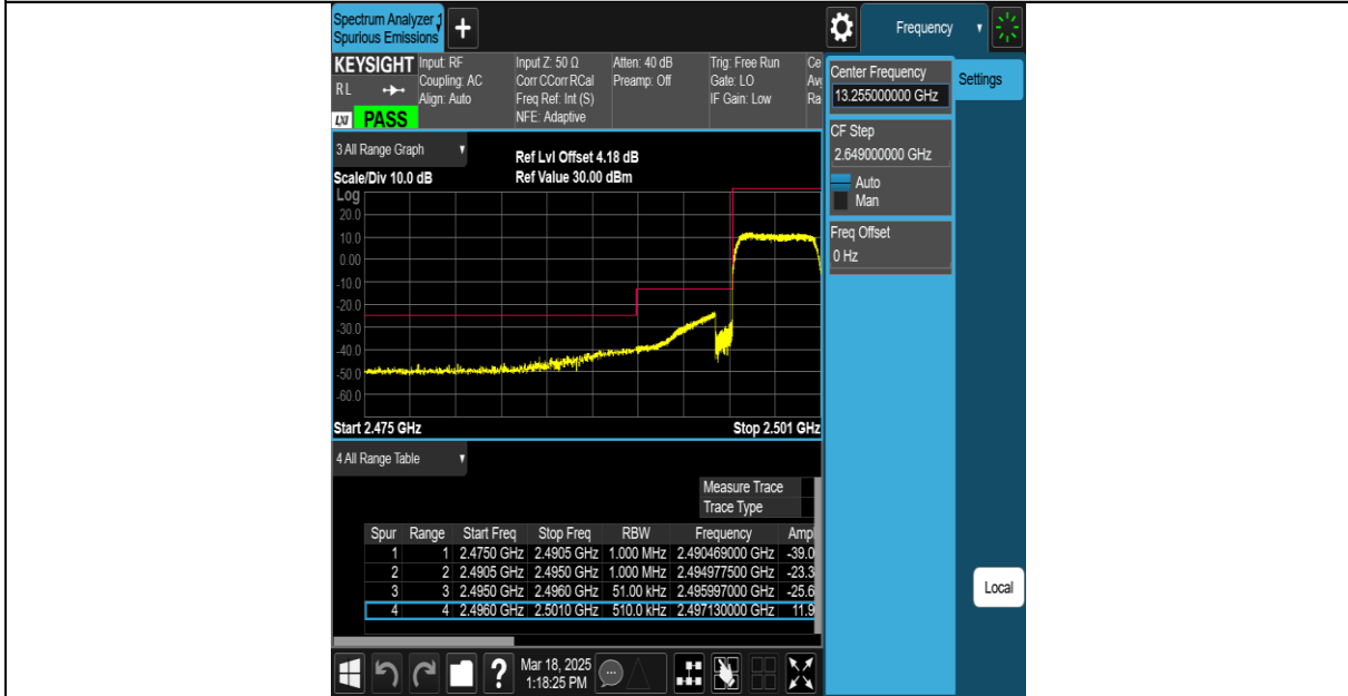
Band41-5MHz-16QAM-41565-25RB#0-PASS
