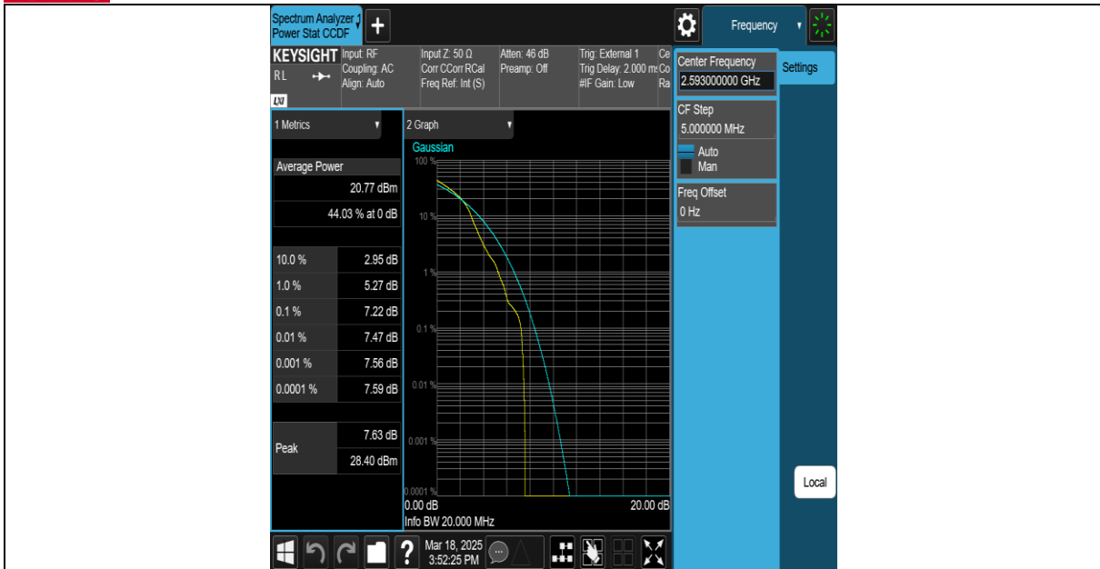
Band41-20MHz-16QAM-40620-27RB#0-PASS
