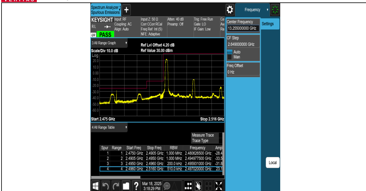
Band41-20MHz-QPSK-39750-100RB#0-PASS
