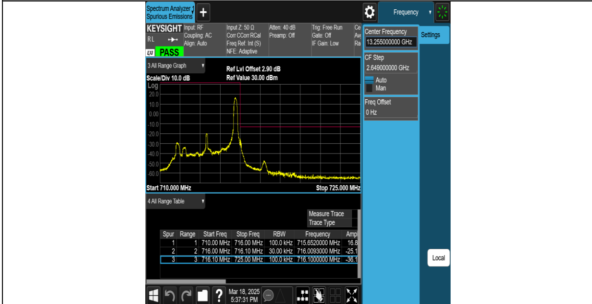
Band12-10MHz-QPSK-23060-1RB#0-PASS
