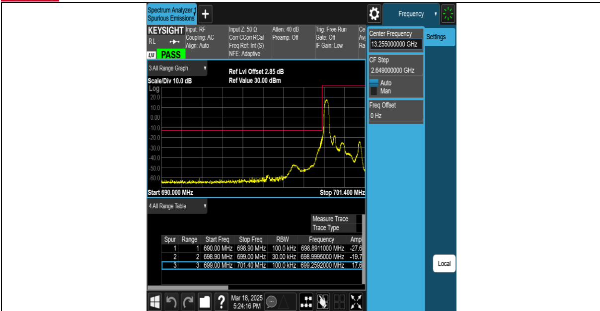
Band12-1.4MHz-16QAM-23017-6RB#0-PASS
