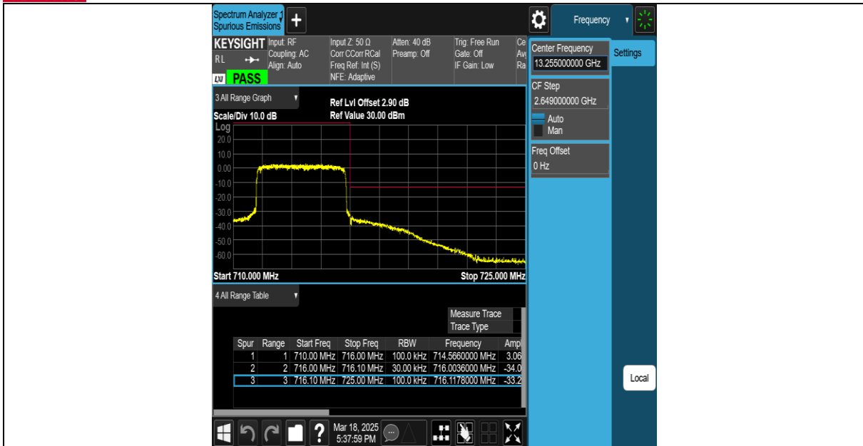
Band12-5MHz-16QAM-23155-1RB#24-PASS
