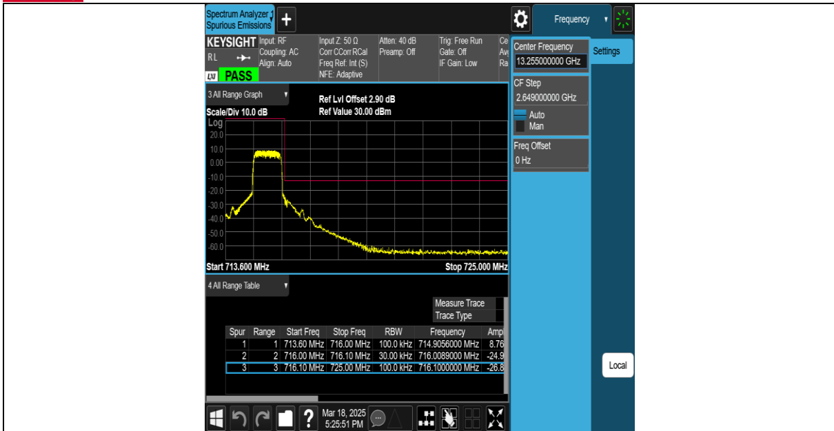
Band12-1.4MHz-16QAM-23173-1RB#5-PASS
