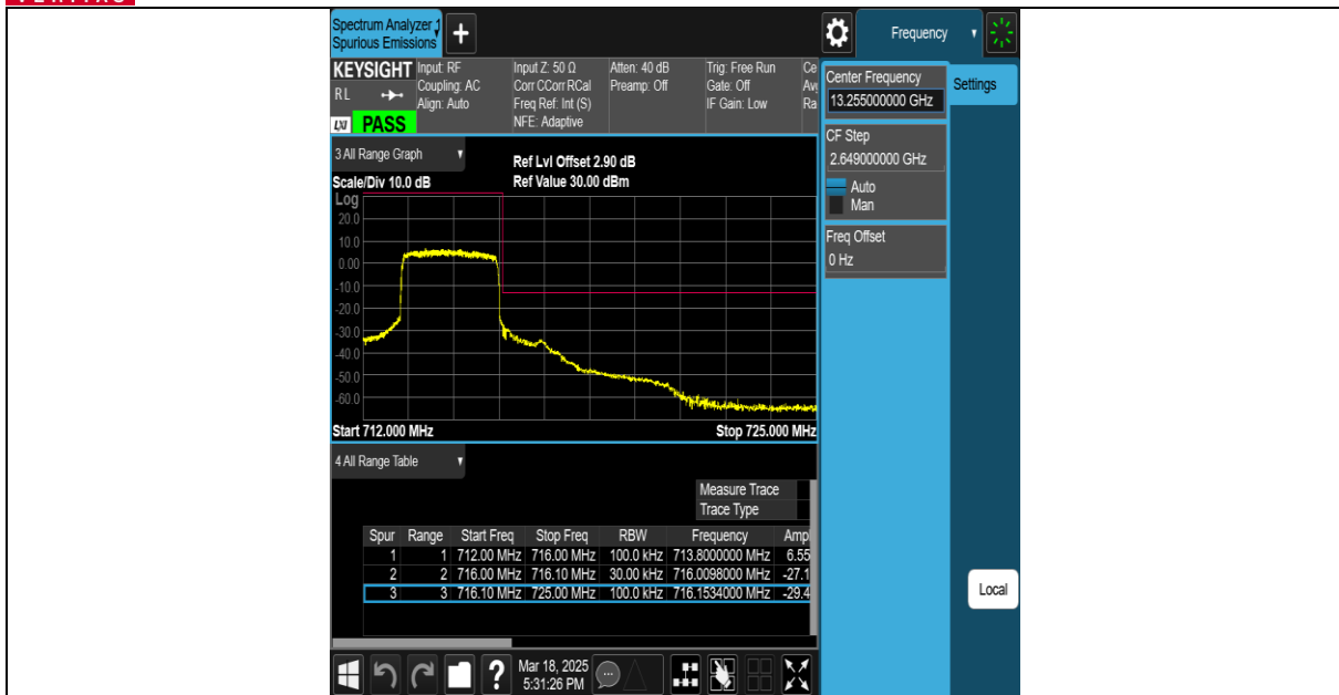
Band12-3MHz-QPSK-23165-1RB#14-PASS
