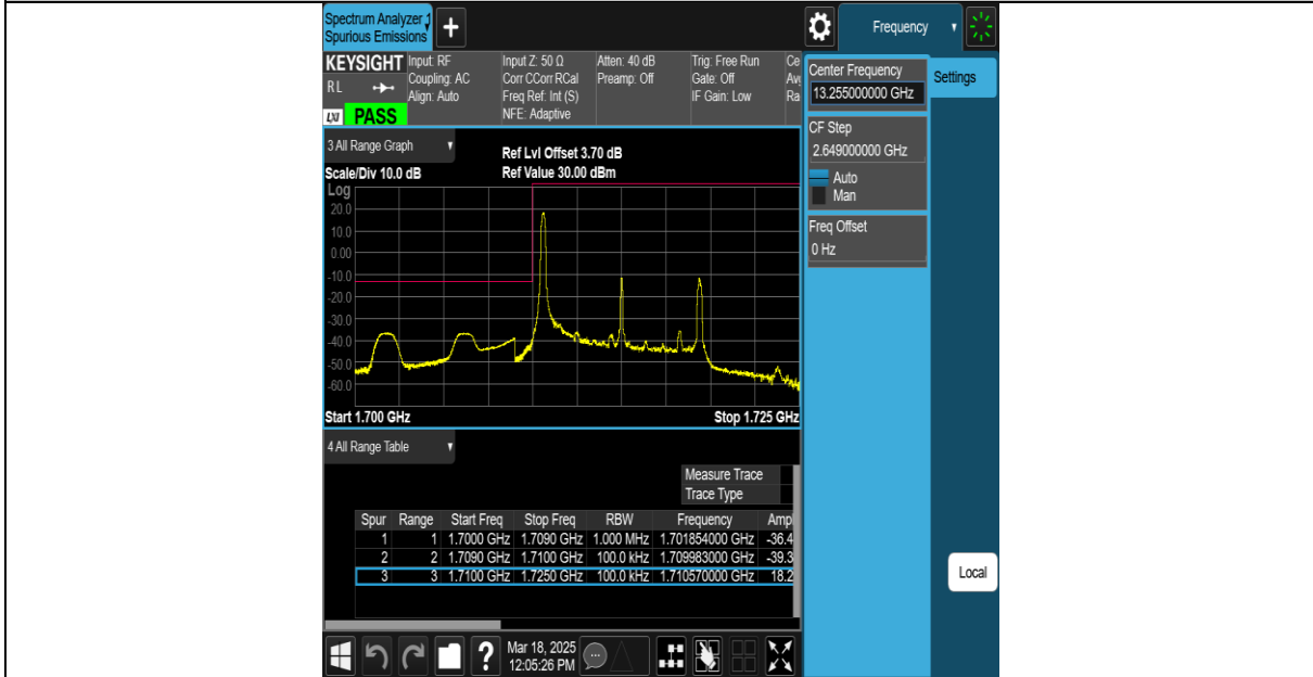
Band66-10MHz-QPSK-132022-50RB#0-PASS
