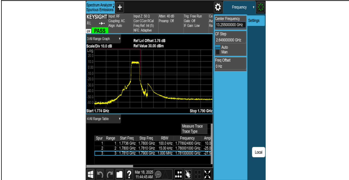
Band66-1.4MHz-QPSK-132665-1RB#5-PASS
