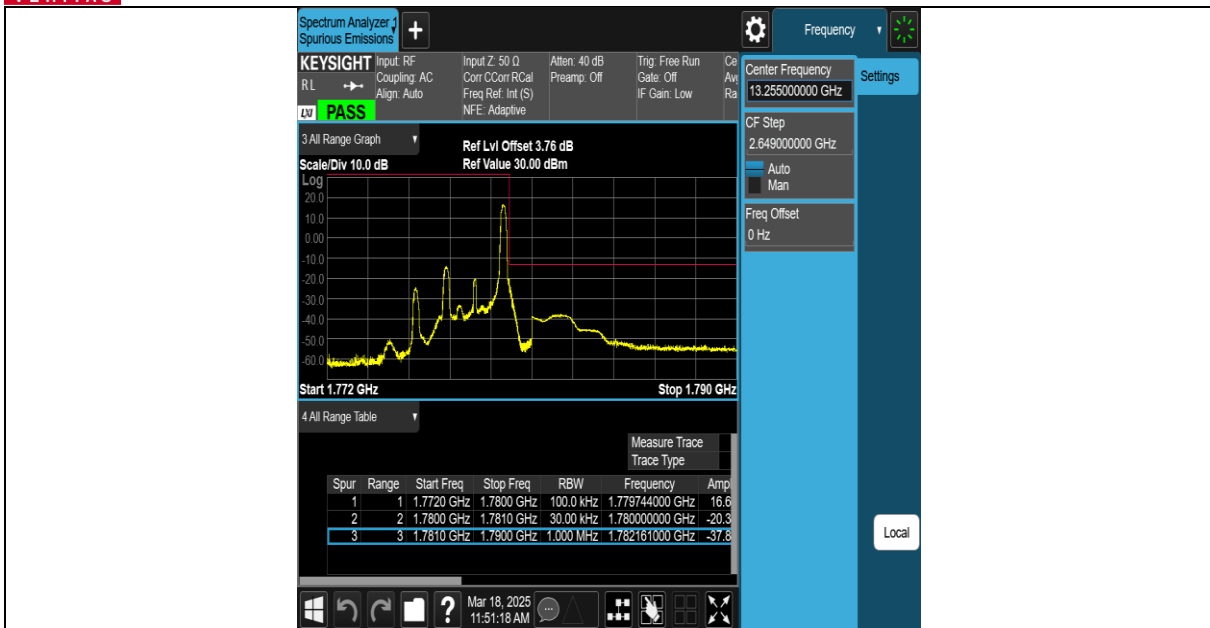
Band66-5MHz-QPSK-131997-1RB#0-PASS
