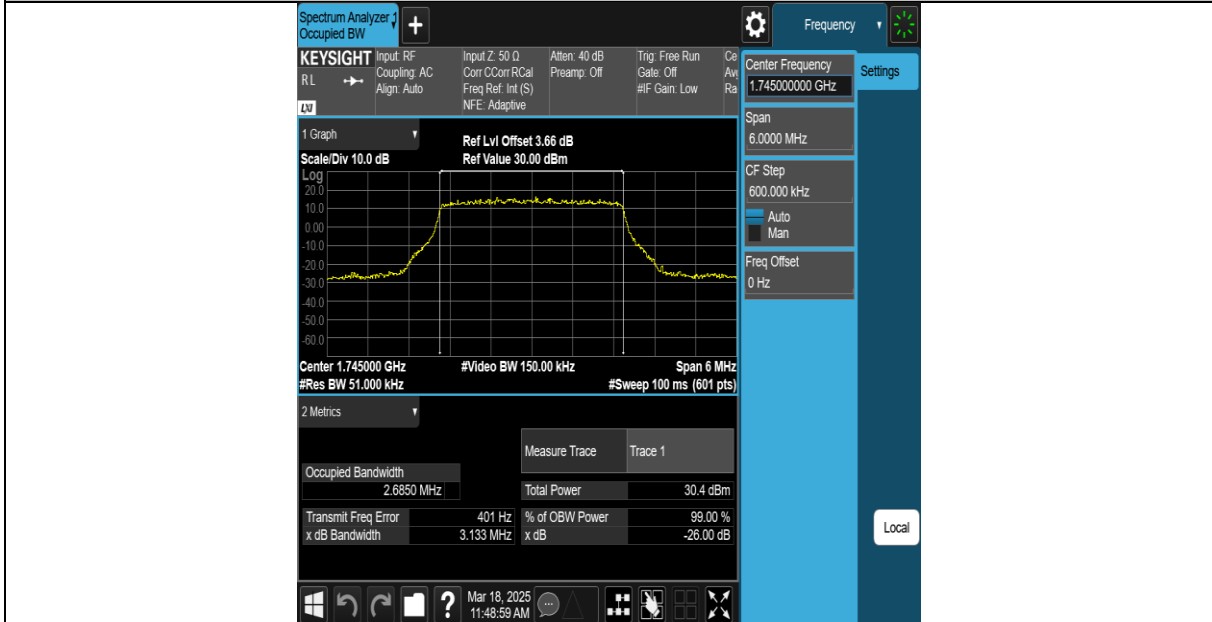
Band66-3MHz-QPSK-132657-15RB#0-PASS
