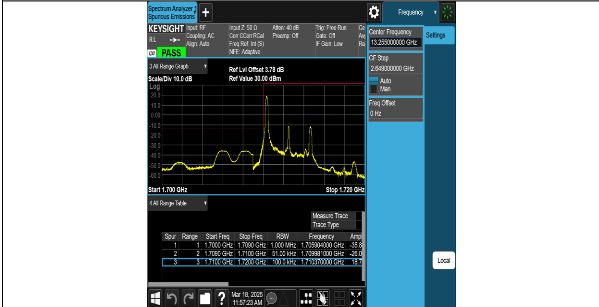
Band66-5MHz-QPSK-131997-25RB#0-PASS
