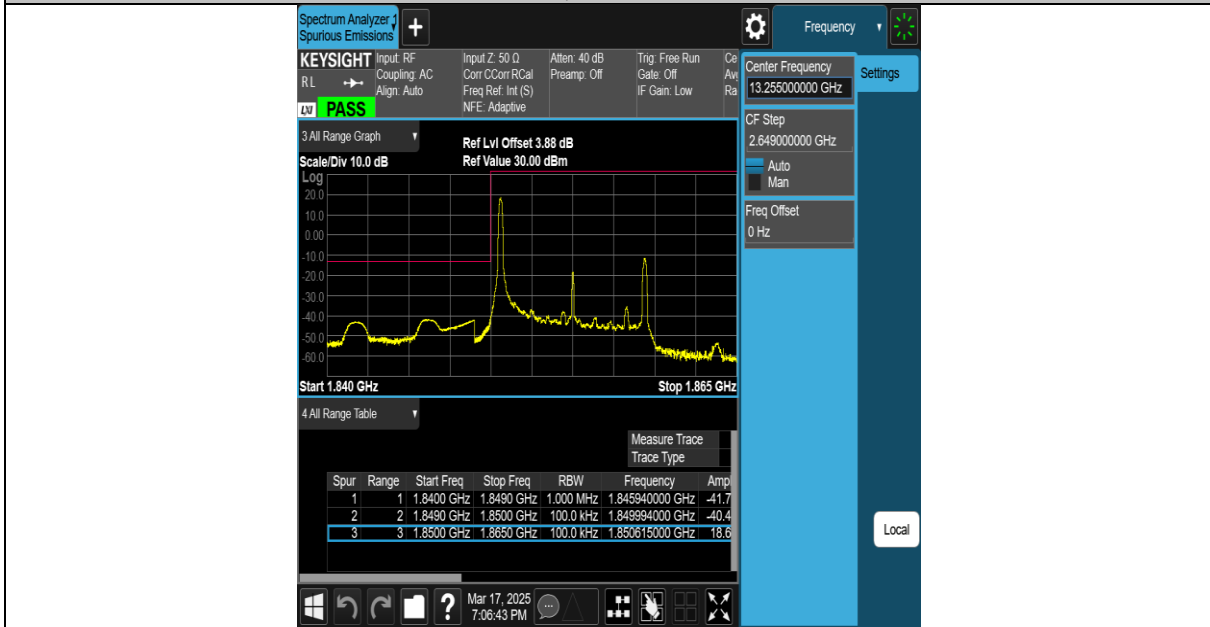
Band25-10MHz-QPSK-26090-50RB#0-PASS
