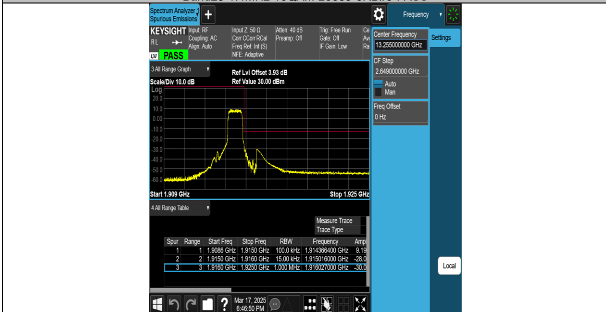
Band25-1.4MHz-16QAM-26683-1RB#5-PASS
