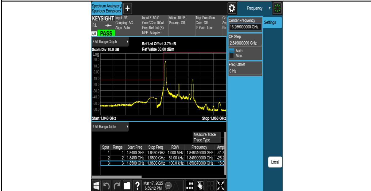
Band25-5MHz-16QAM-26065-25RB#0-PASS
