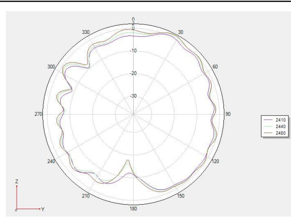
WIF/BT: 2440Mhz
