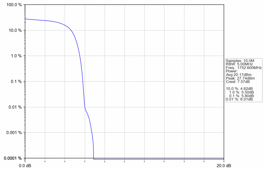
Band4_HSDPA_HCH_1752.6MHz_Subtest 1_NTNV
