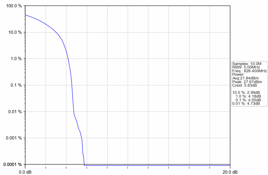
Band5_HSUPA_LCH_826.4MHz_Subtest 1_NTNV
