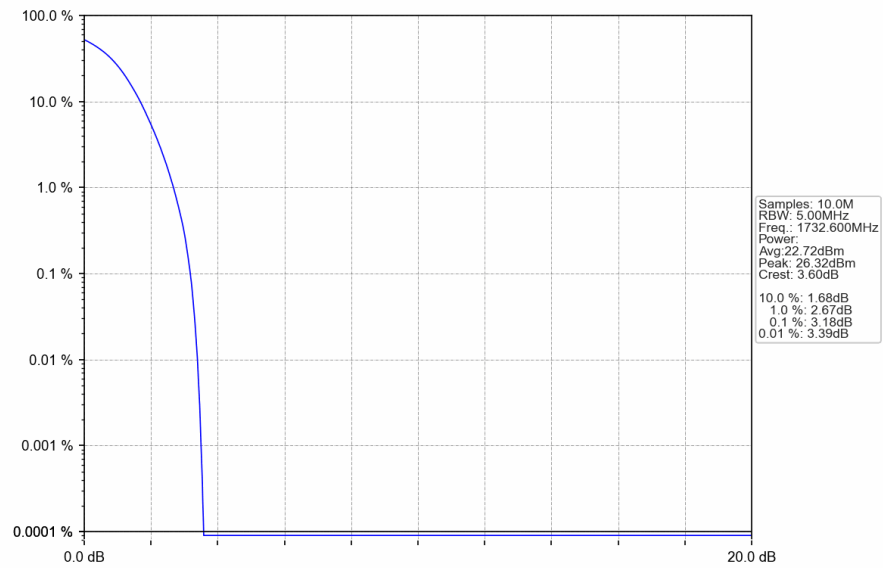
Band4_HSUPA_MCH_1732.6MHz_Subtest 1_NTNV
