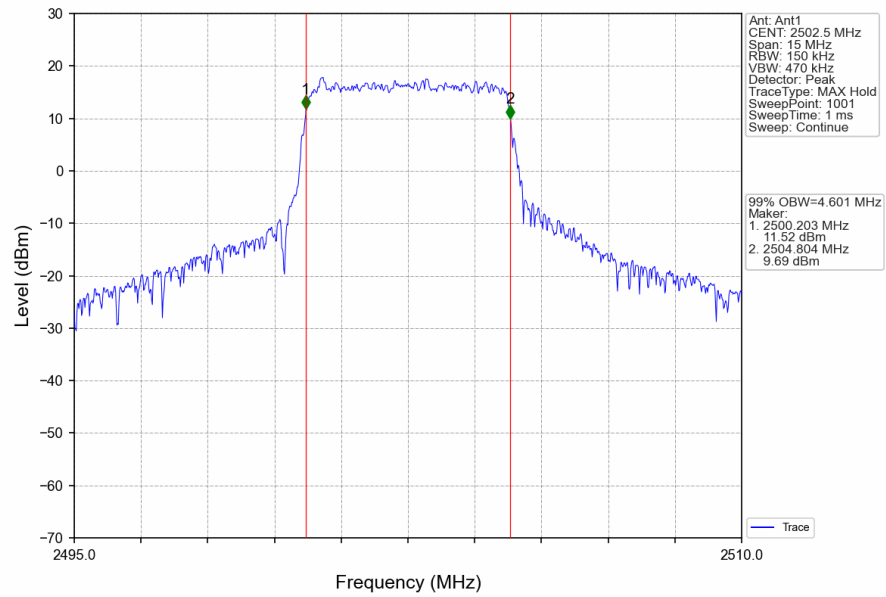
Band7_5MHz_16QAM_LCH_2502.5MHz_RB_25_0_NTNV
