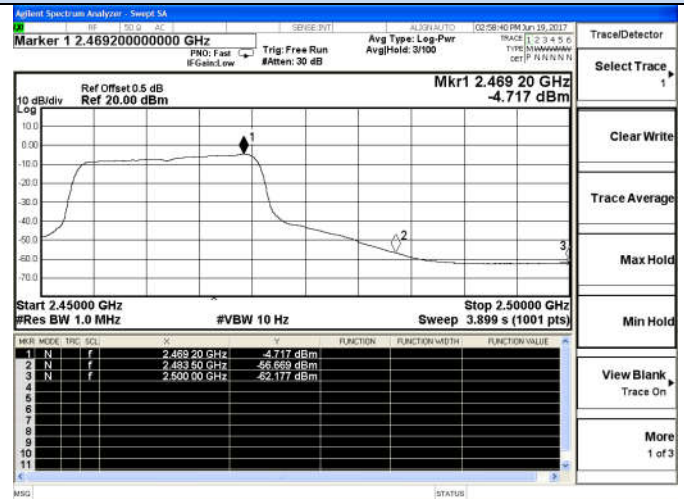
802.11g-High channel(Average)
