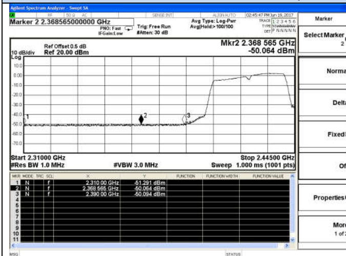
802.11n(HT40)-Low channel(Peak)
