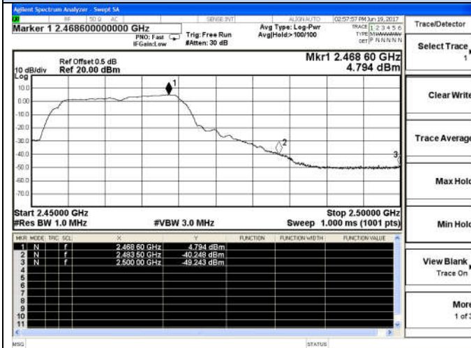
802.11g-High channel(Peak)
