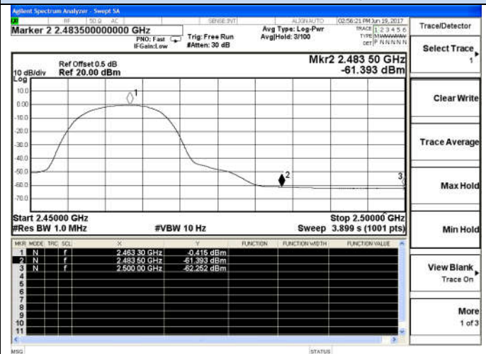
802.11b-High channel(Average)
