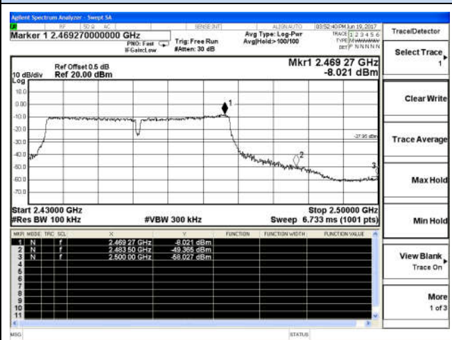
Channel 9 / 2452 MHz
