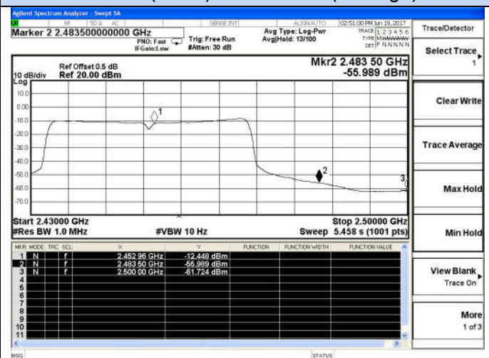
802.11n(HT40)-High channel(Average)
