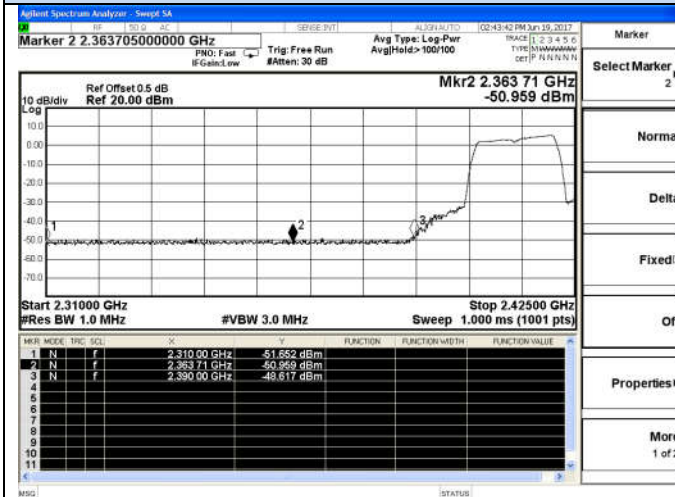
802.11n(HT20)-Low channel(Peak)
