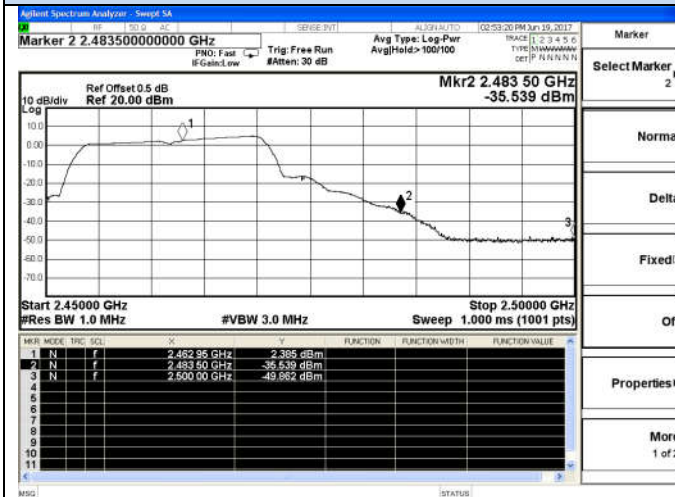
802.11n(HT20)-High channel(Peak)
