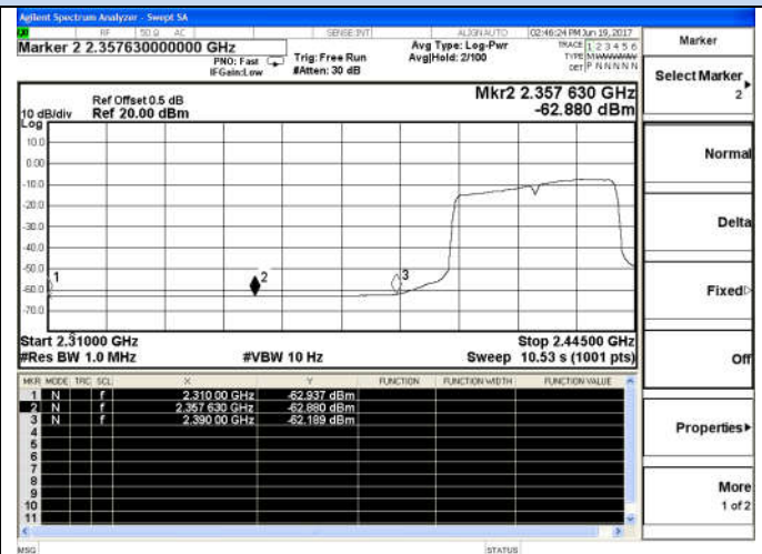
802.11n(HT40)-Low channel(Average)
