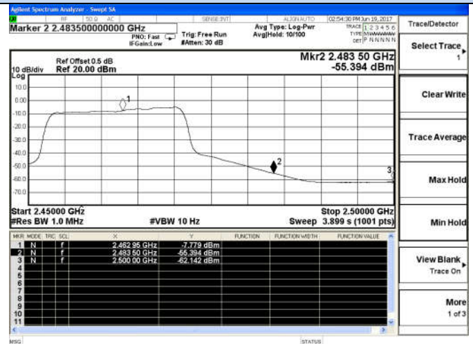
802.11n(HT20)-High channel(Average)
