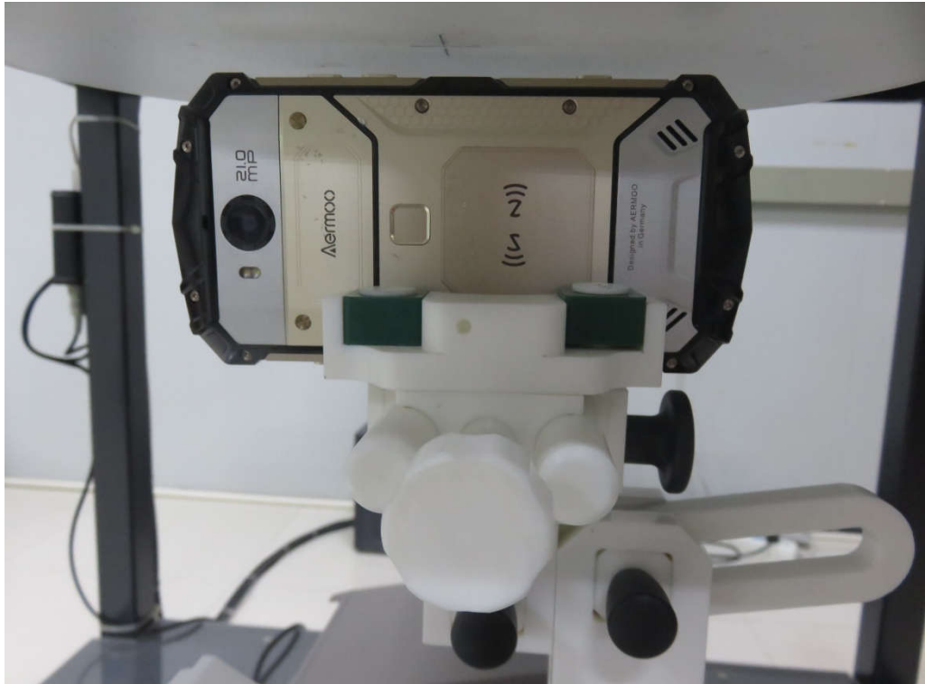
10mm body-worn Left Side Setup Photo(hotspot)
