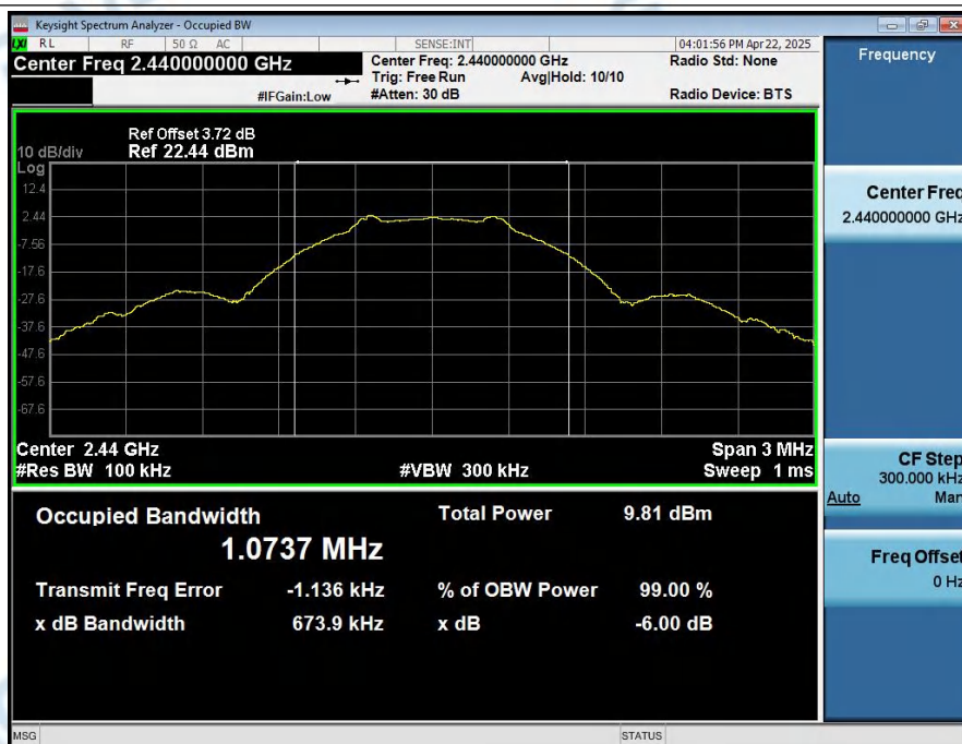
-6dB_Bandwidth_NVNT_ANT1_1Mbps_2440
