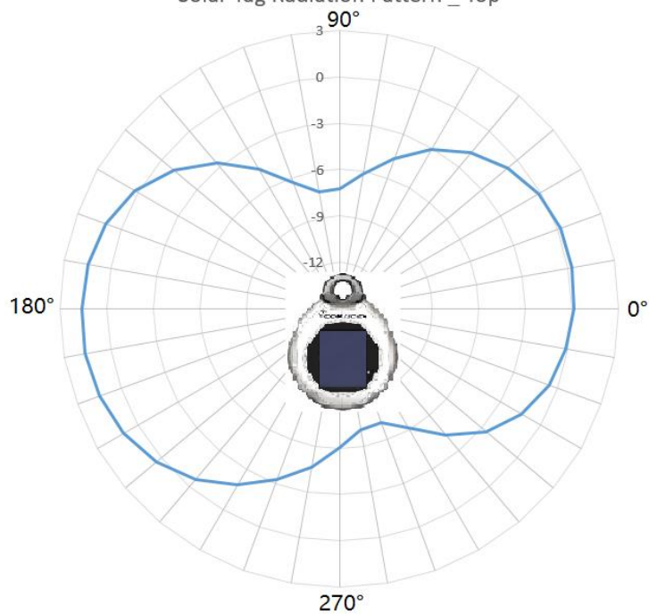
Solar Tag Radiation Pattern _ Top
