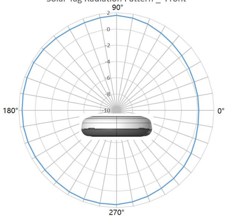
Solar Tag Radiation Pattern _ Front
