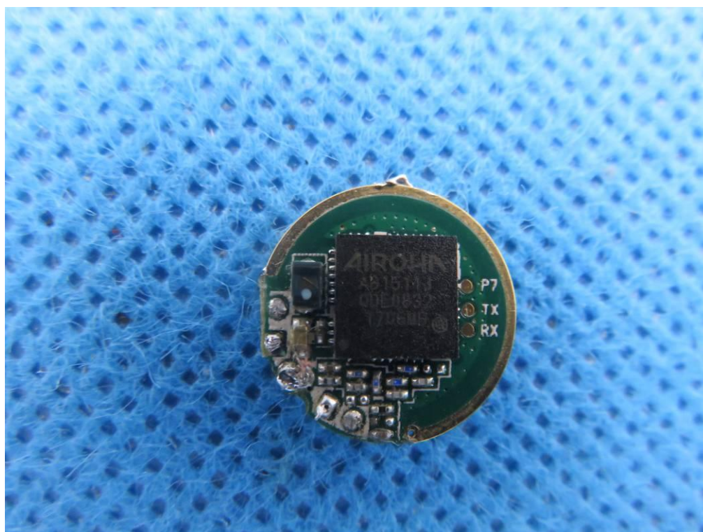
INTERNAL VIEW OF EUT-7 (Left)
