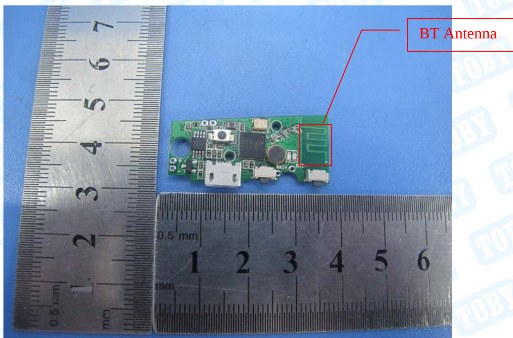
Photo 11 Appearance of PCB
