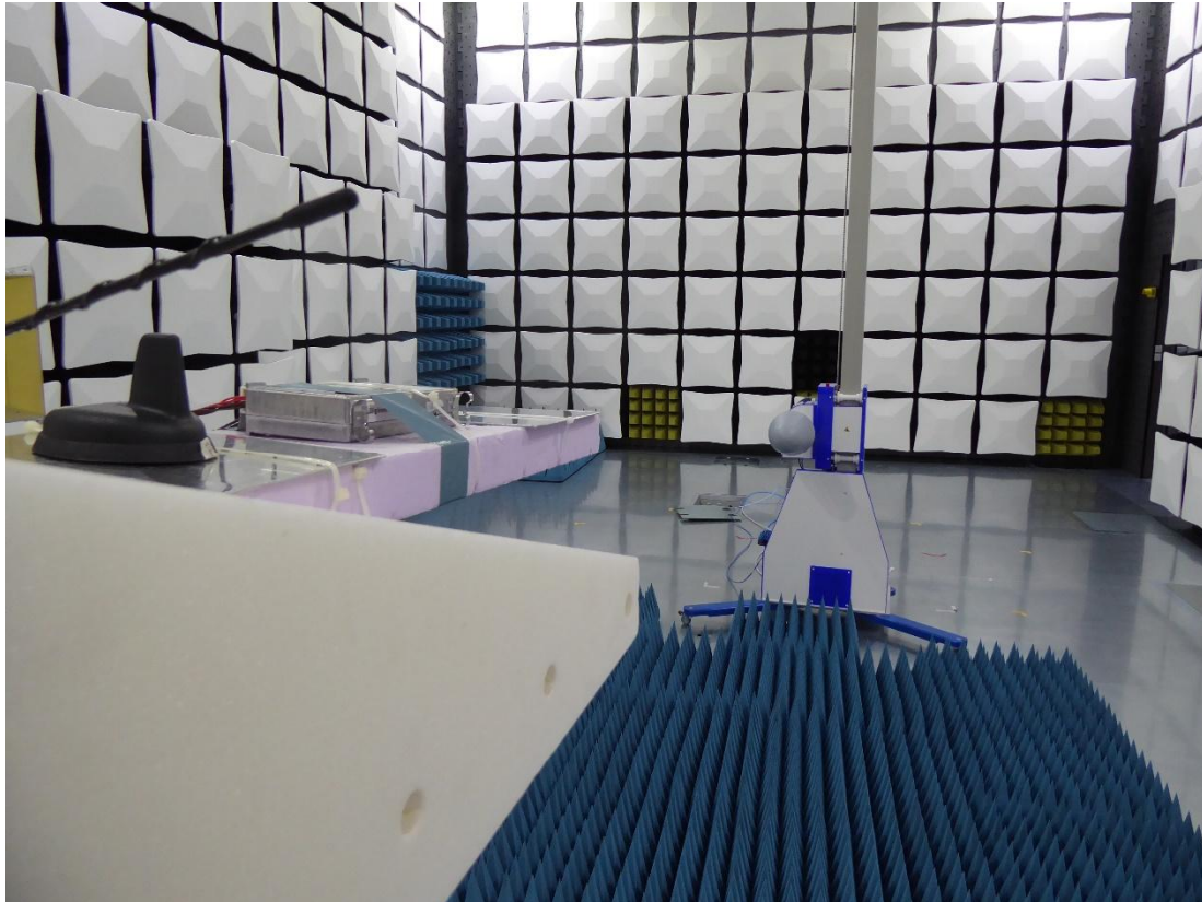
191350_4.JPG: Test setup 1 - 18 GHz
