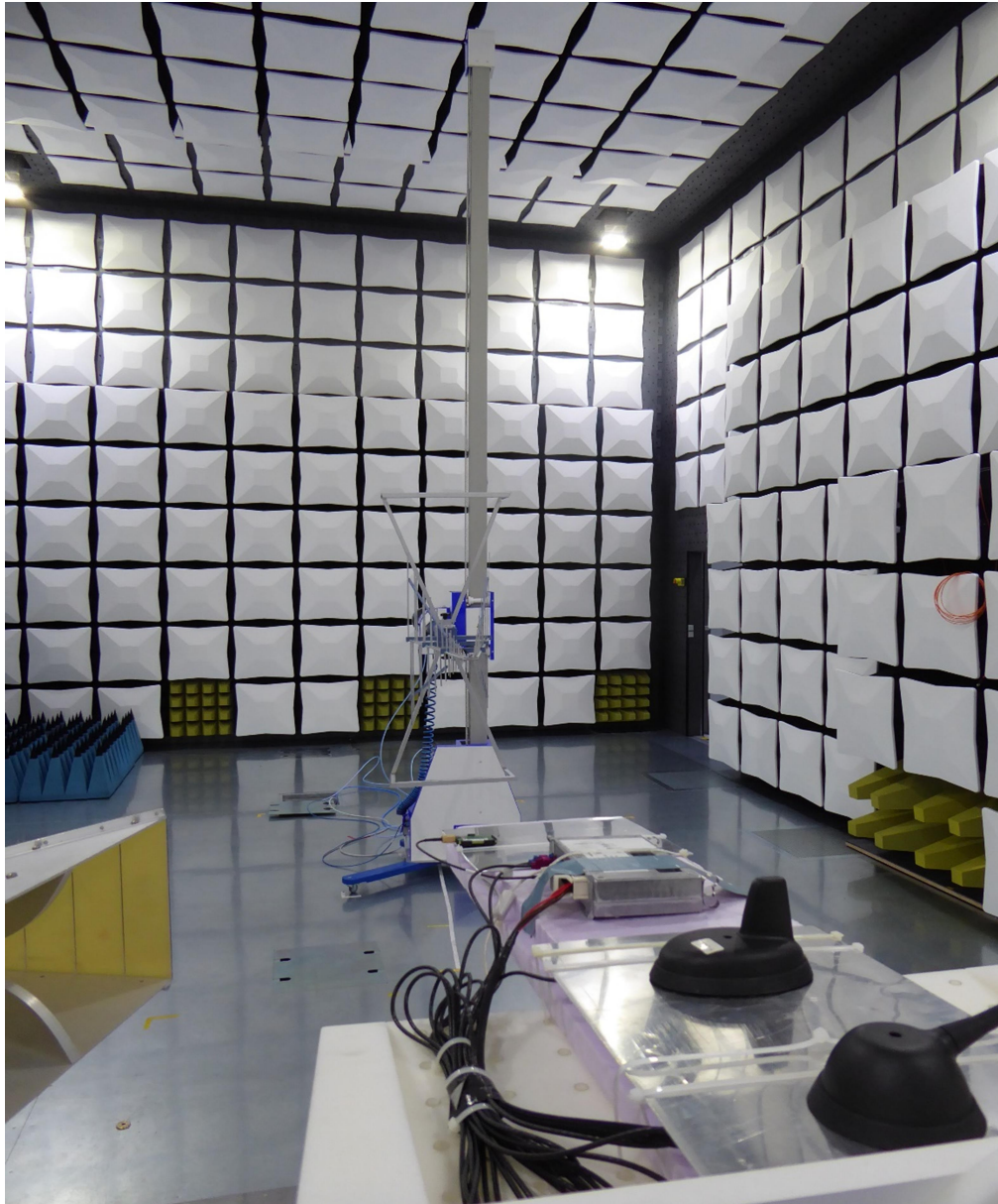
191350_3.JPG: Test setup below 1 GHz
