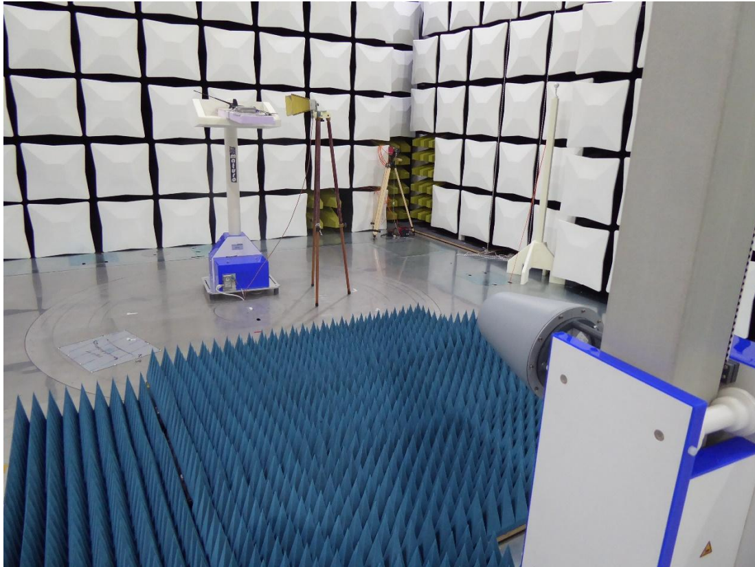
191350_5.JPG: Test setup 1 - 18GHz
