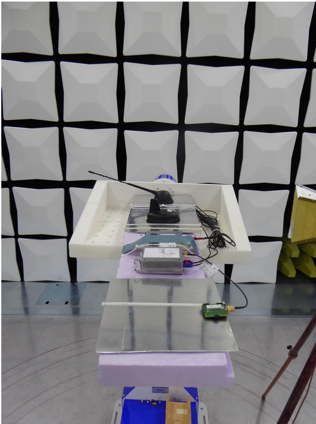
191350_1.JPG: Test setup on positioner
