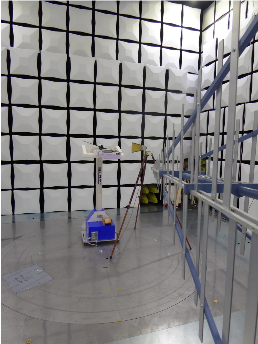
191350_2.JPG: Test setup below 1 GHz
