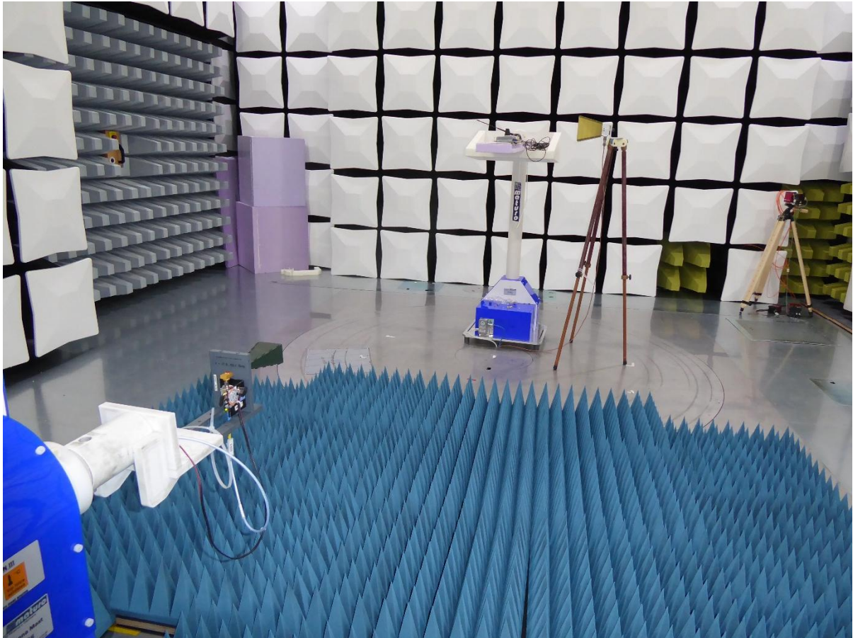
191350_6.JPG: Test setup 18 – 26.5 GHz
