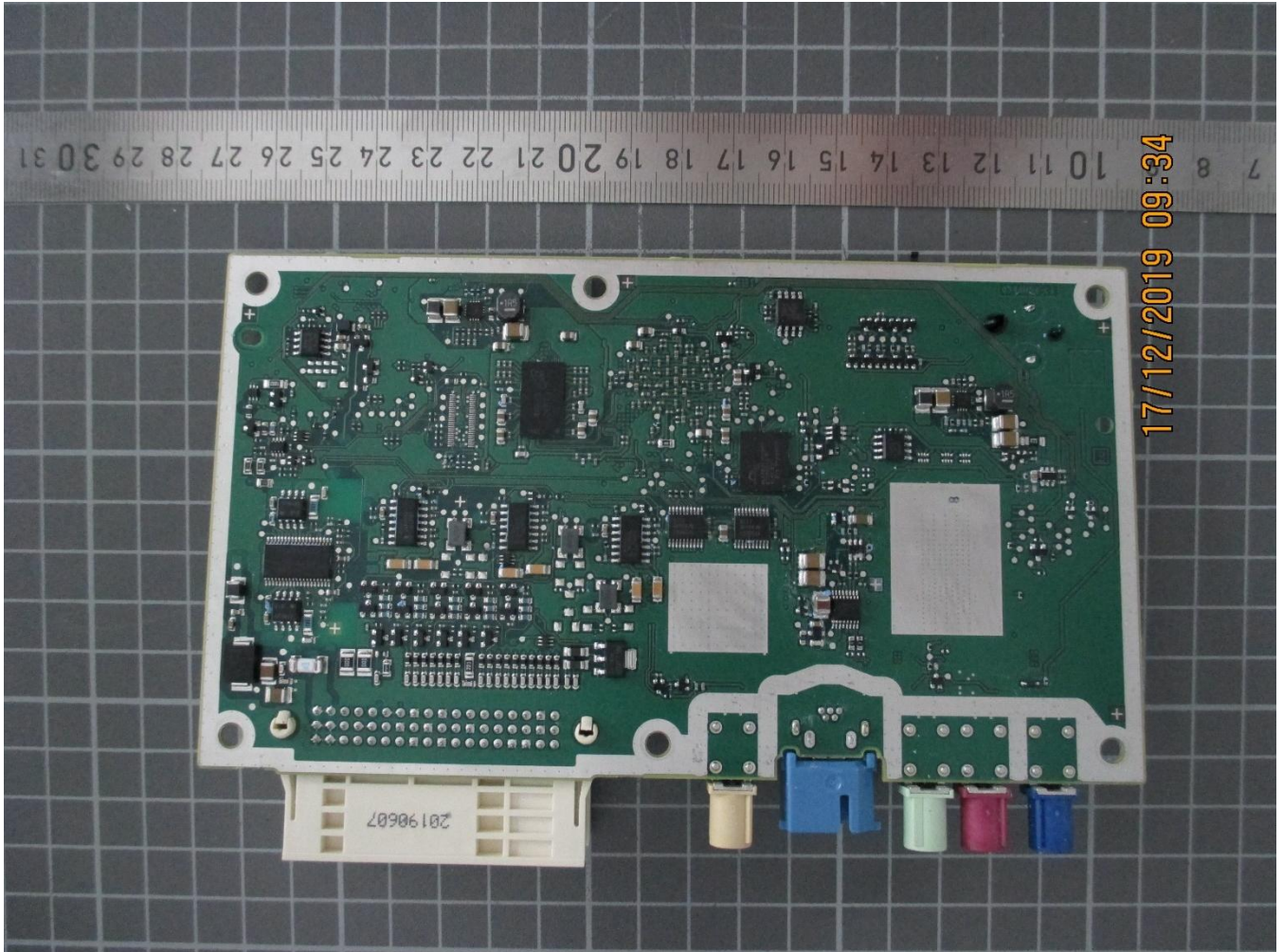
191350_14.JPG: PCB Bottom view
