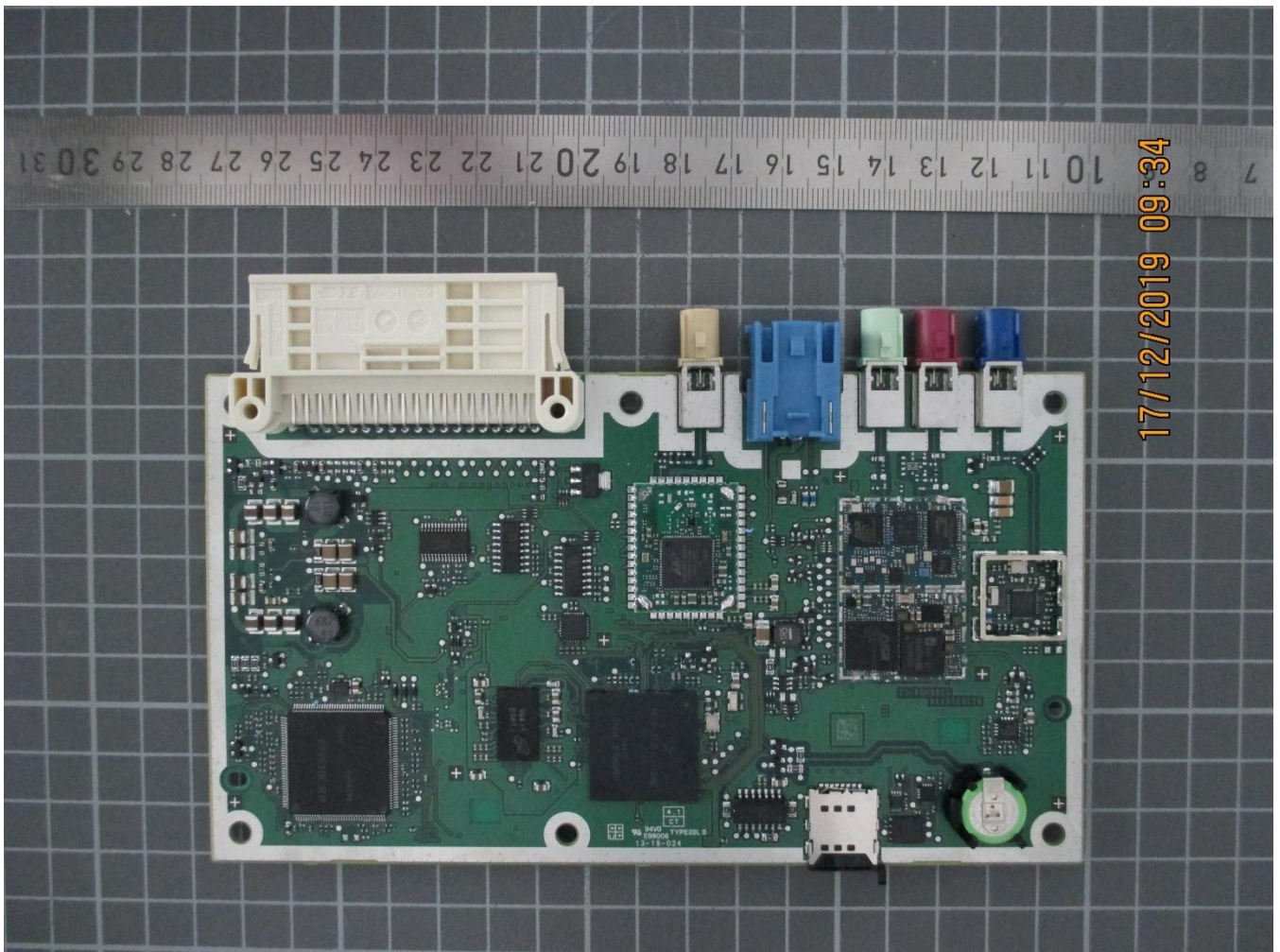
191350_13.JPG: PCB Top view
