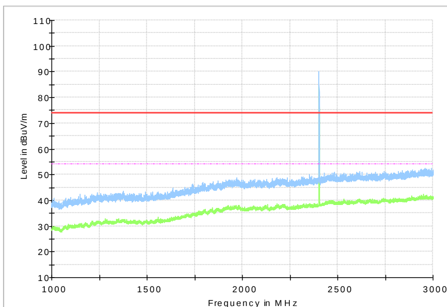
Fig.88 Radiated Spurious Emission (8DPSK, Ch0, 1GHz ~3GHz , Vertical Direction)
