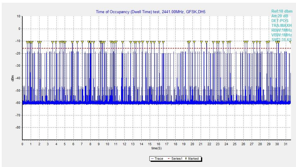
Fig. 109 Time of Occupancy(Dwell Time) (GFSK, Ch39)
