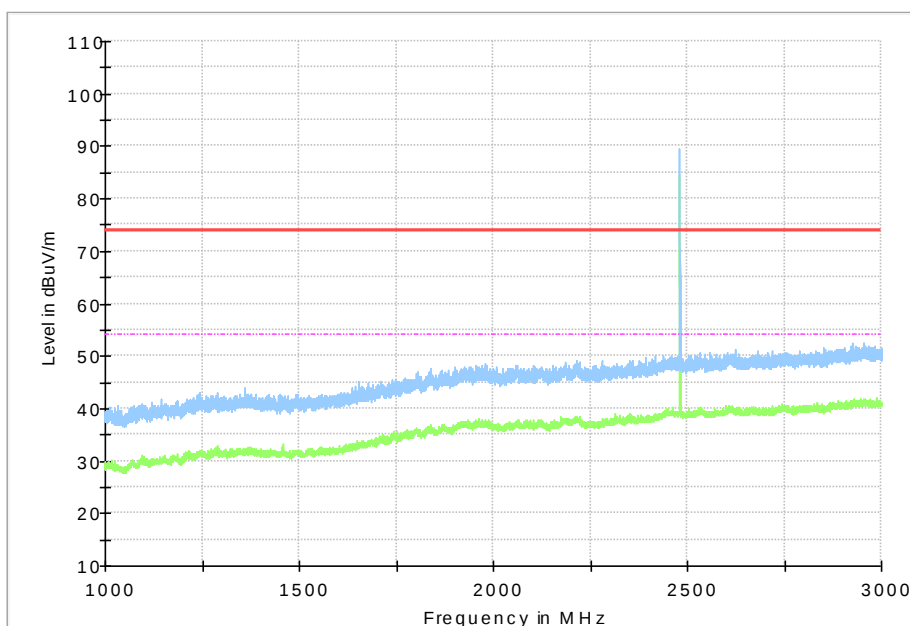
Fig.84 Radiated Spurious Emission (8DPSK, Ch78, 1GHz ~3 GHz ,Horizontal Direction)
