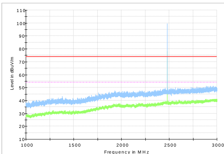
Fig.46 Radiated Spurious Emission (GFSK, Ch78, 1GHz ~3 GHz ,Horizontal Direction)
