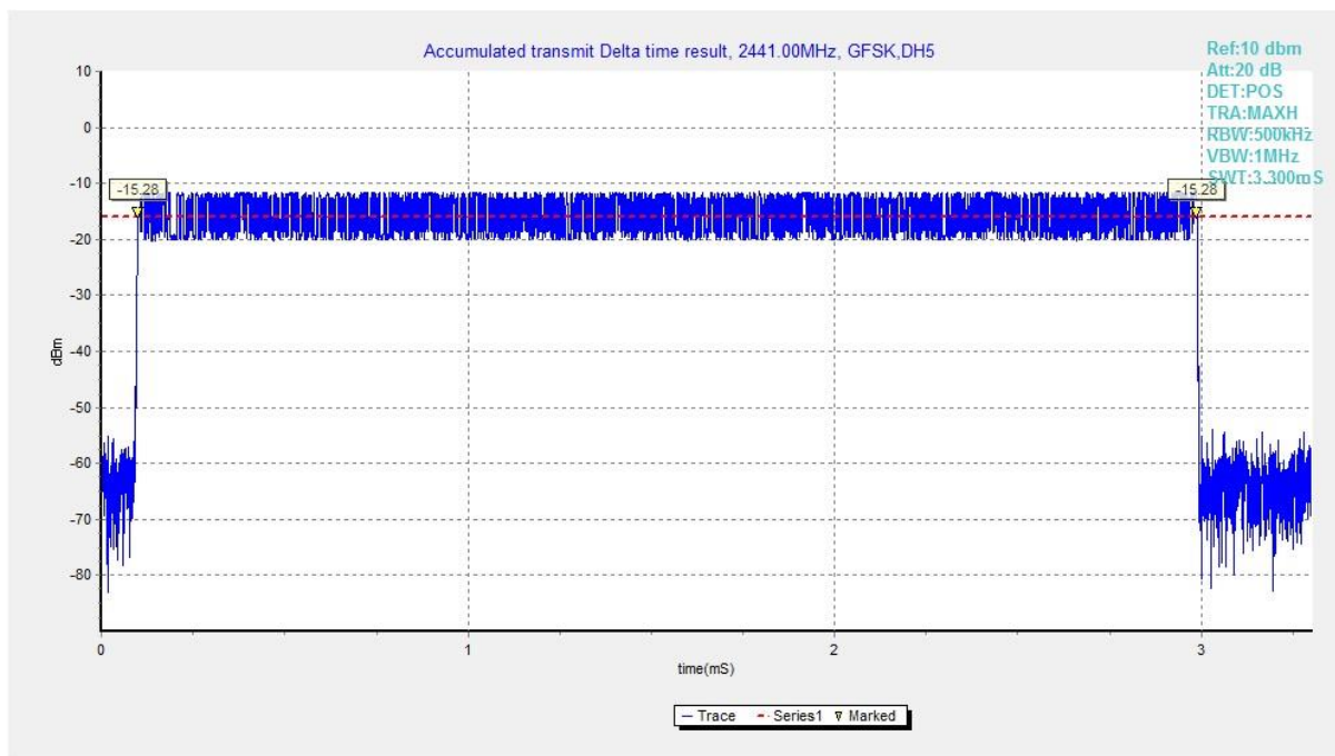
Fig. 108 Time of Occupancy(Dwell Time) (GFSK, Ch39)
