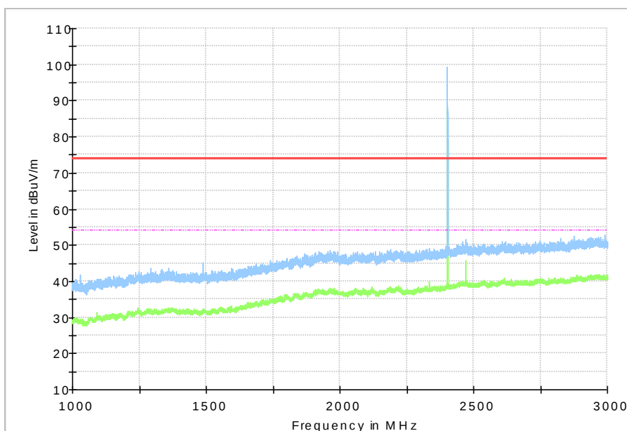
Fig.50 Radiated Spurious Emission (GFSK, Ch0, 1GHz ~3GHz , Vertical Direction)
