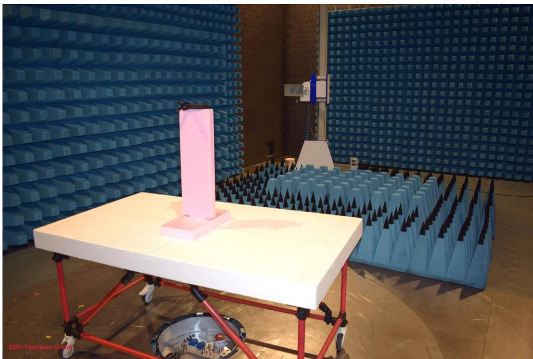
Picture 5: EUT test setup radiated emission test from 1 GHz to 10th harmonic (front view)
