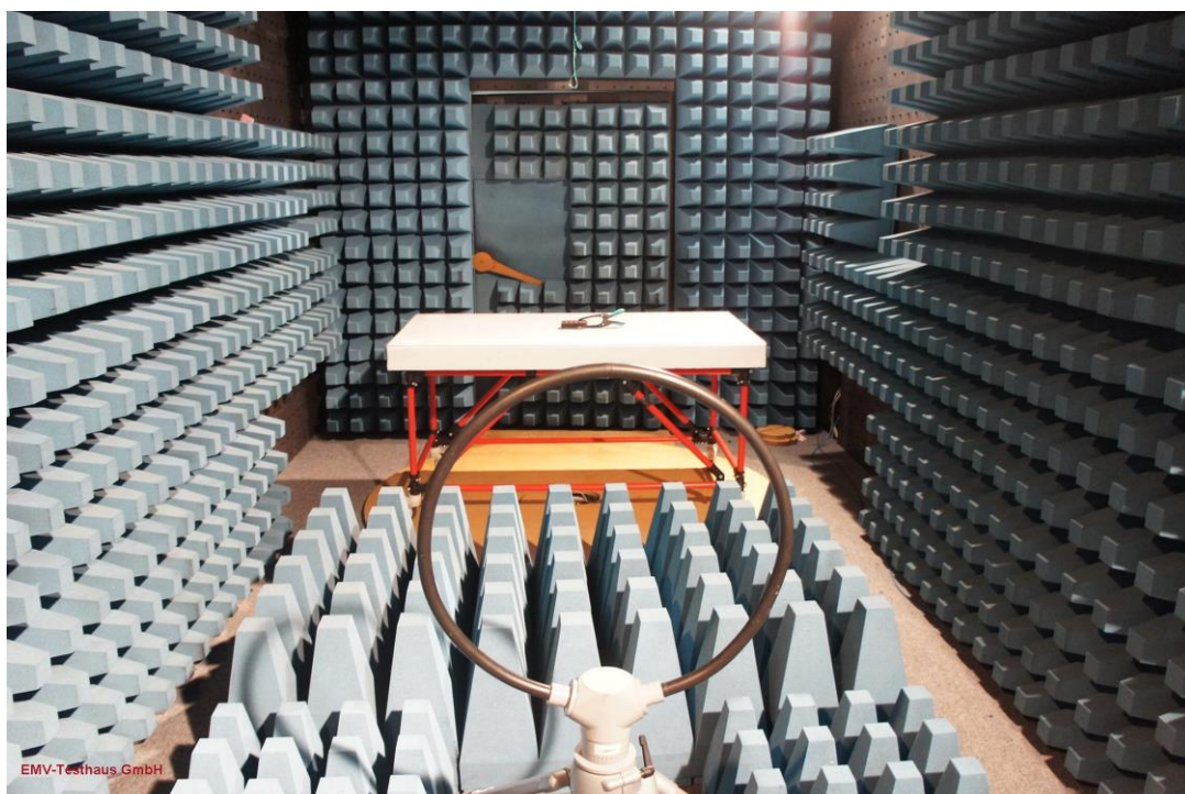
Picture 2: EUT test setup radiated emission test below 30 MHz (rear view)
