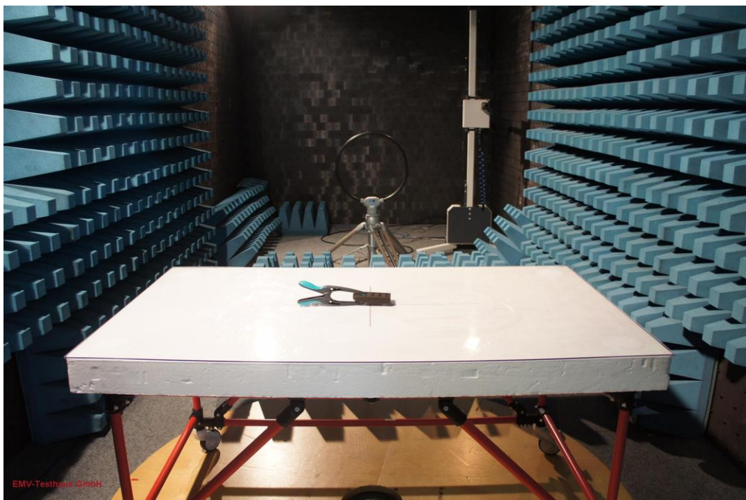
Picture 1: EUT test setup radiated emission test below 30 MHz (front view)
