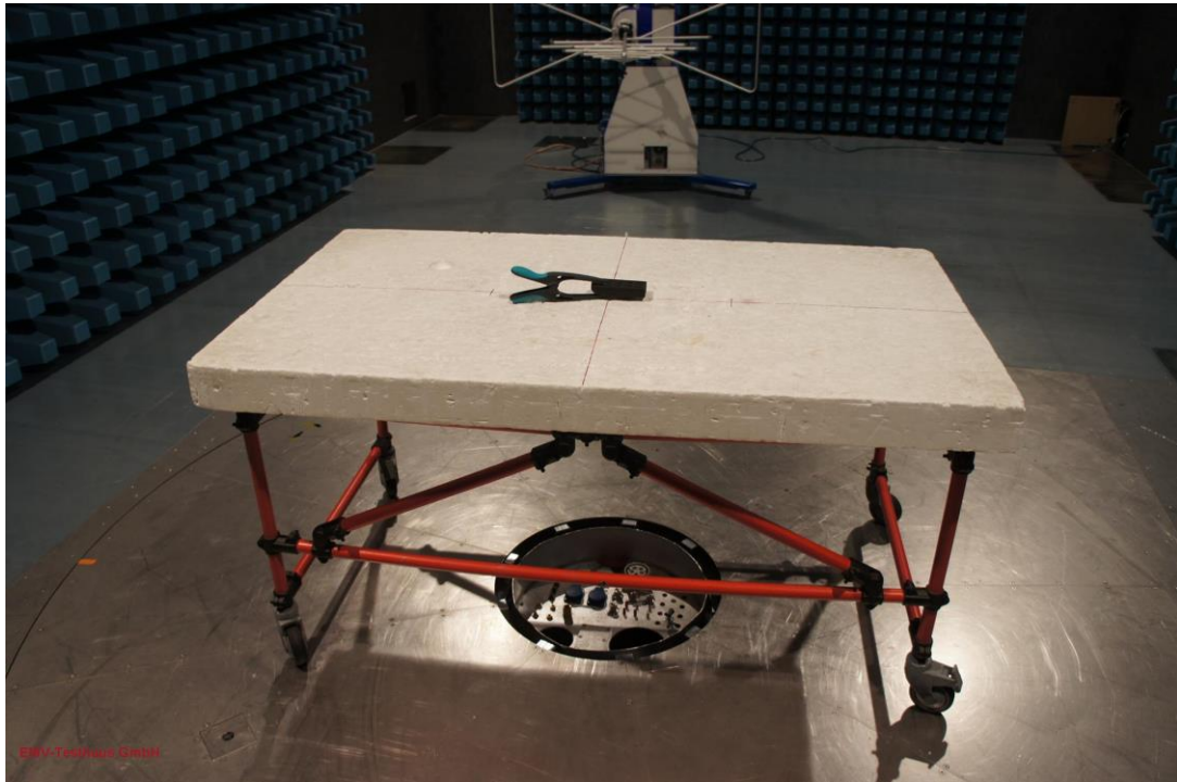
Picture 3: EUT test setup radiated emission test from 30 MHz to 1 GHz (front view)
