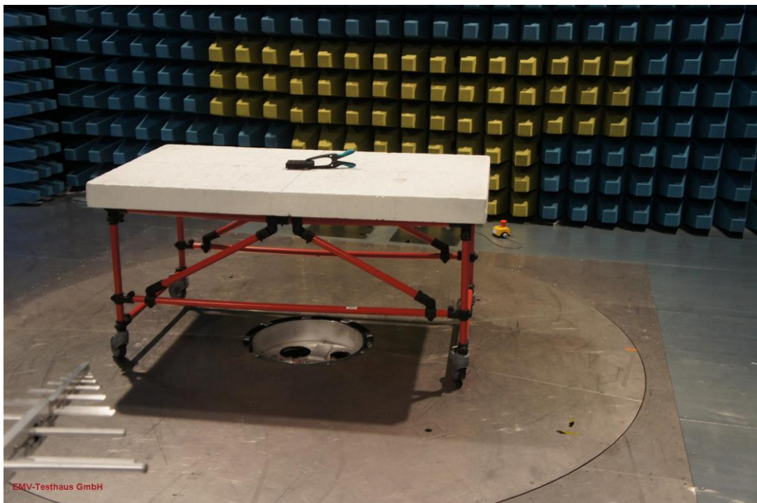
Picture 4: EUT test setup radiated emission test from 30 MHz to 1 GHz (rear view)
