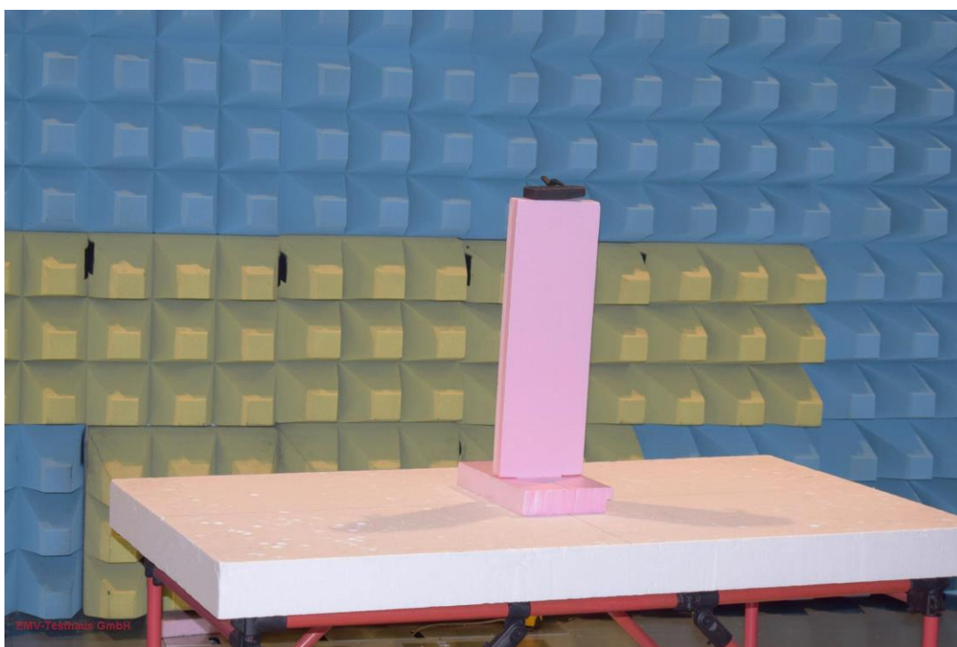
Picture 6: EUT test setup radiated emission test from 1 GHz to 10th harmonic (rear view)
