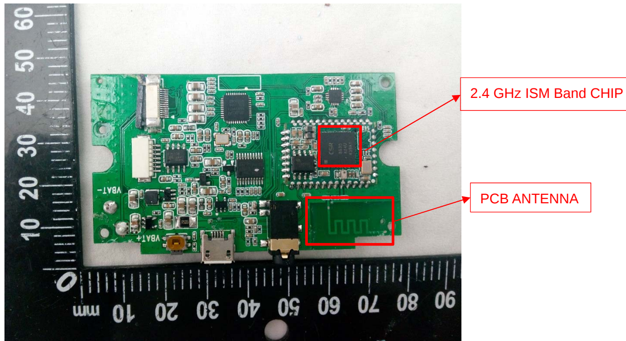
MAIN BOARD 2 TOP VIEW
