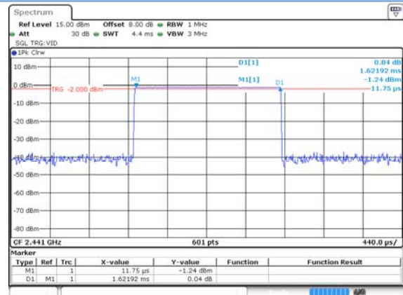
GFSK DH3
