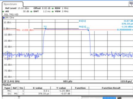
GFSK DH1
