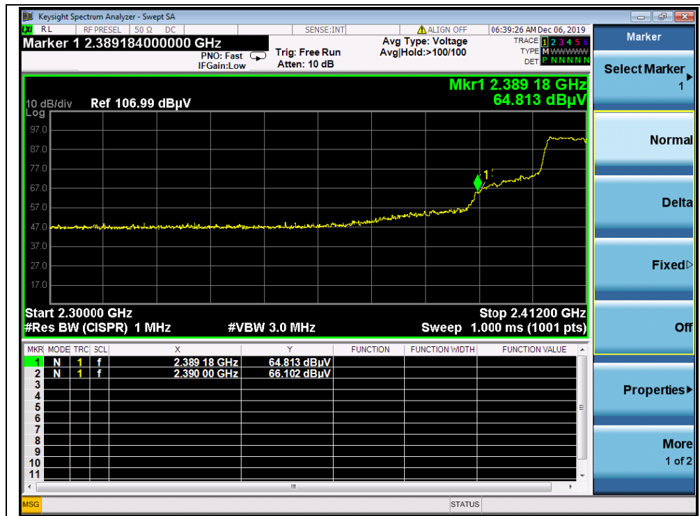
(PEAK, Channel 1, 802.11n (HT20))
