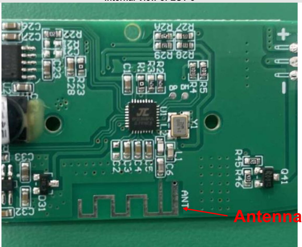
Internal View of EUT-5
