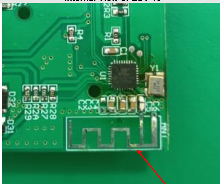
Internal View of EUT-10
