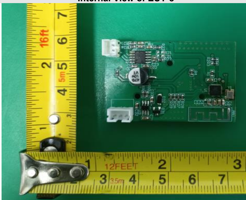
Internal View of EUT-8
