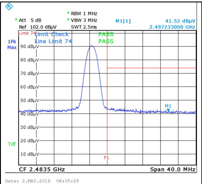
GFSK-Right Side-PK
