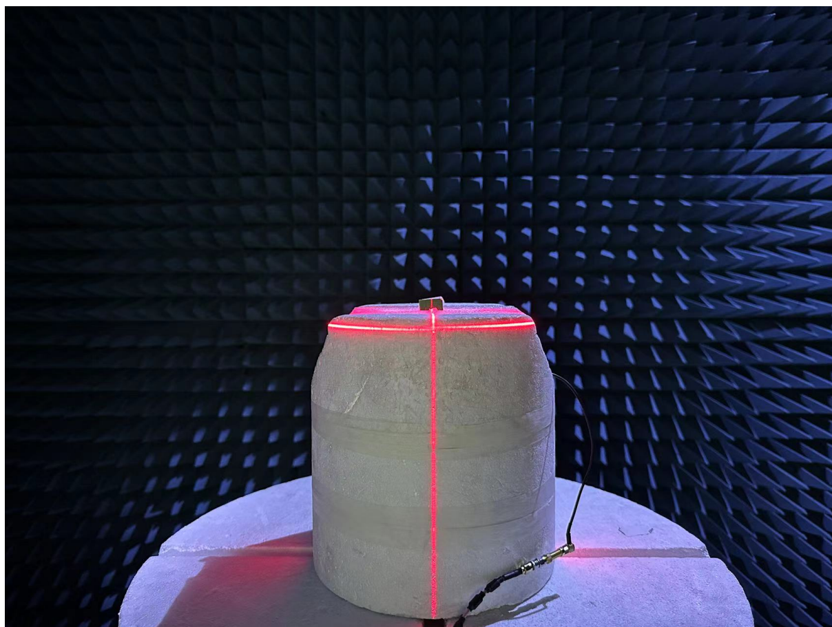
Free Space View of EUT
