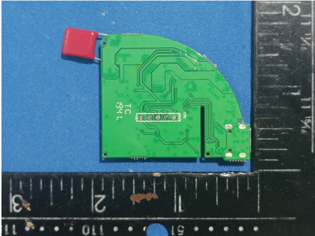
Coil Antenna
