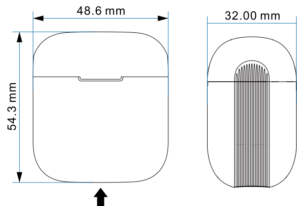
Charging Interface
