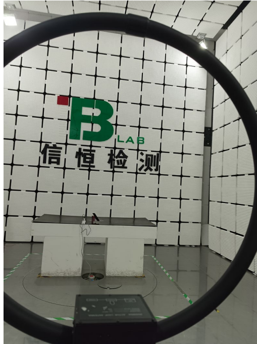
Radiated Emission (9 kHz -30MHz)
