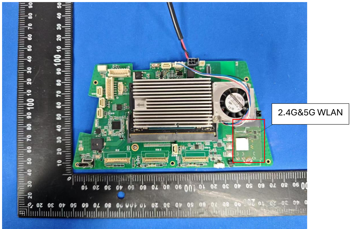
Internal View 7
