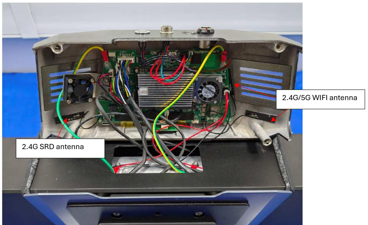
Internal View 2
