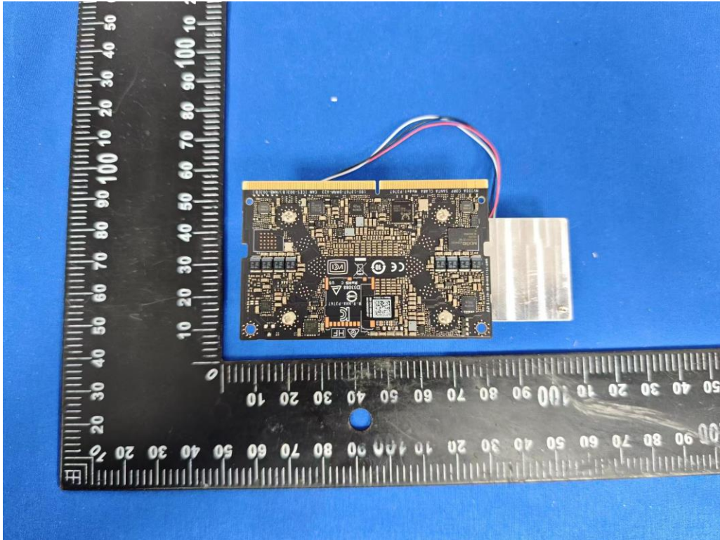
Internal View 5
