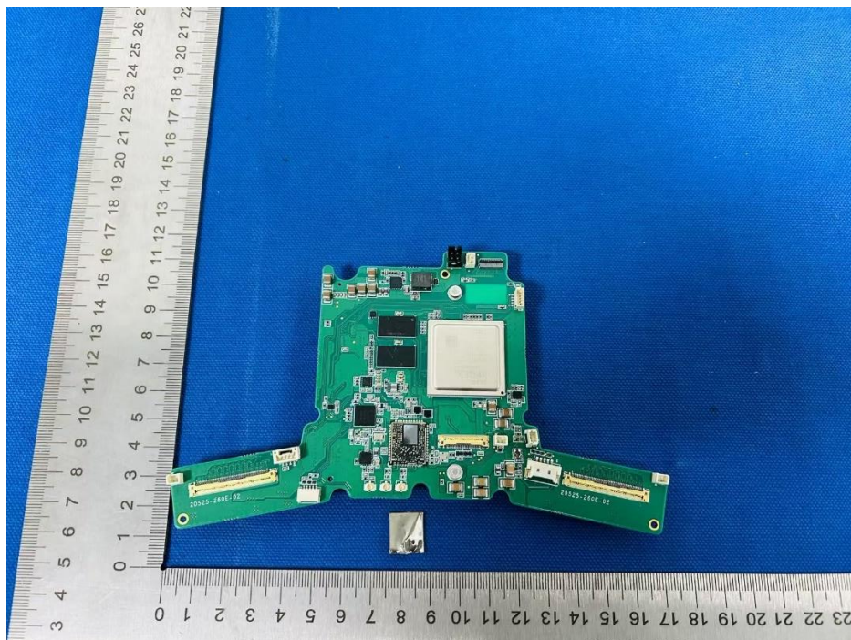
Internal View 6 (Wi-Fi Chip Shield-off)
