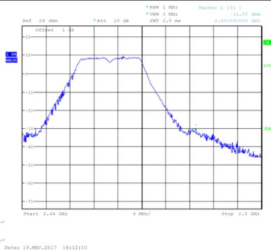
2462 MHz – Peak
