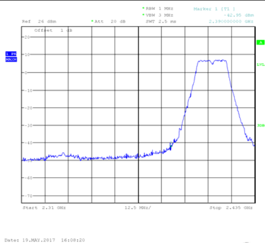
2412 MHz – Peak
