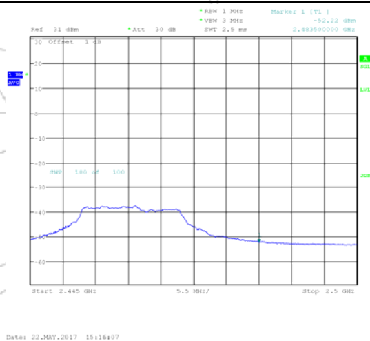
2462 MHz – Average
