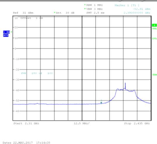
2412 MHz – Average
