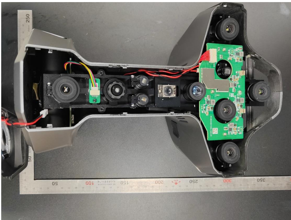
Internal View 2
