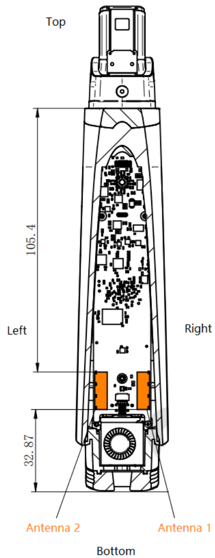
Figure 1.1-1 Antenna Locations (Front view)
