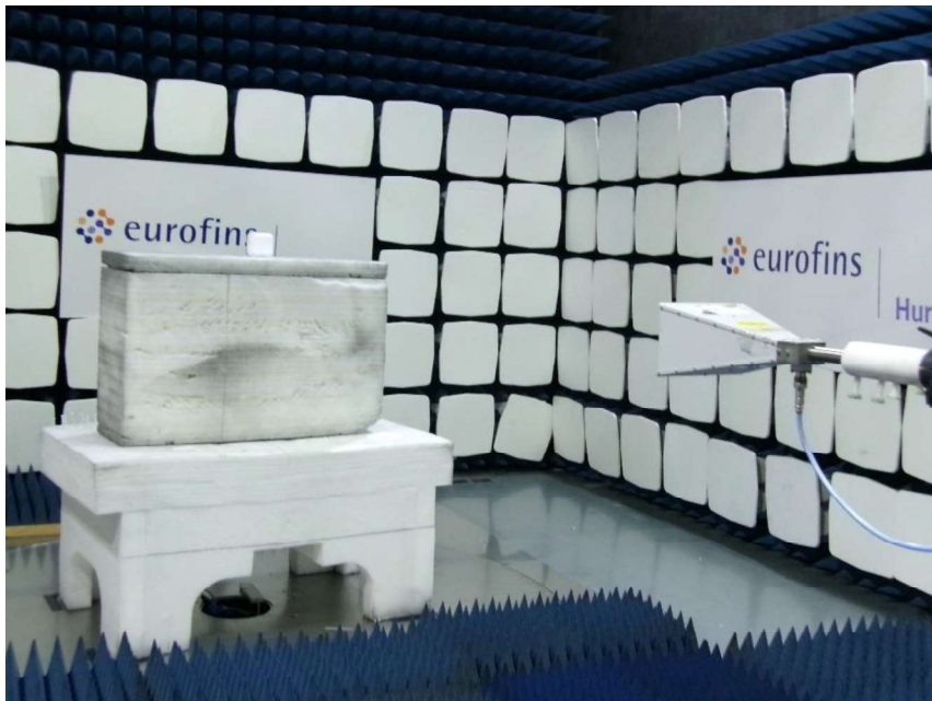
Radiated Emissions; Above 1.0 GHz X-Orientation
