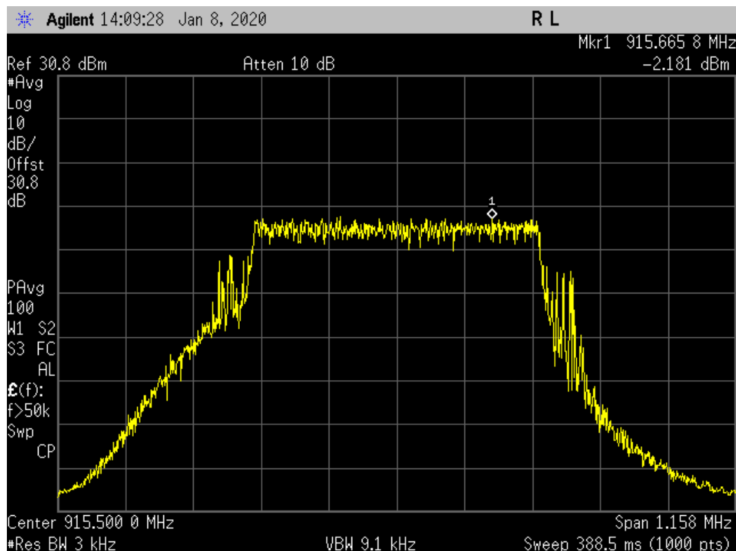
Plot for Power Spectral Density (PSD)
