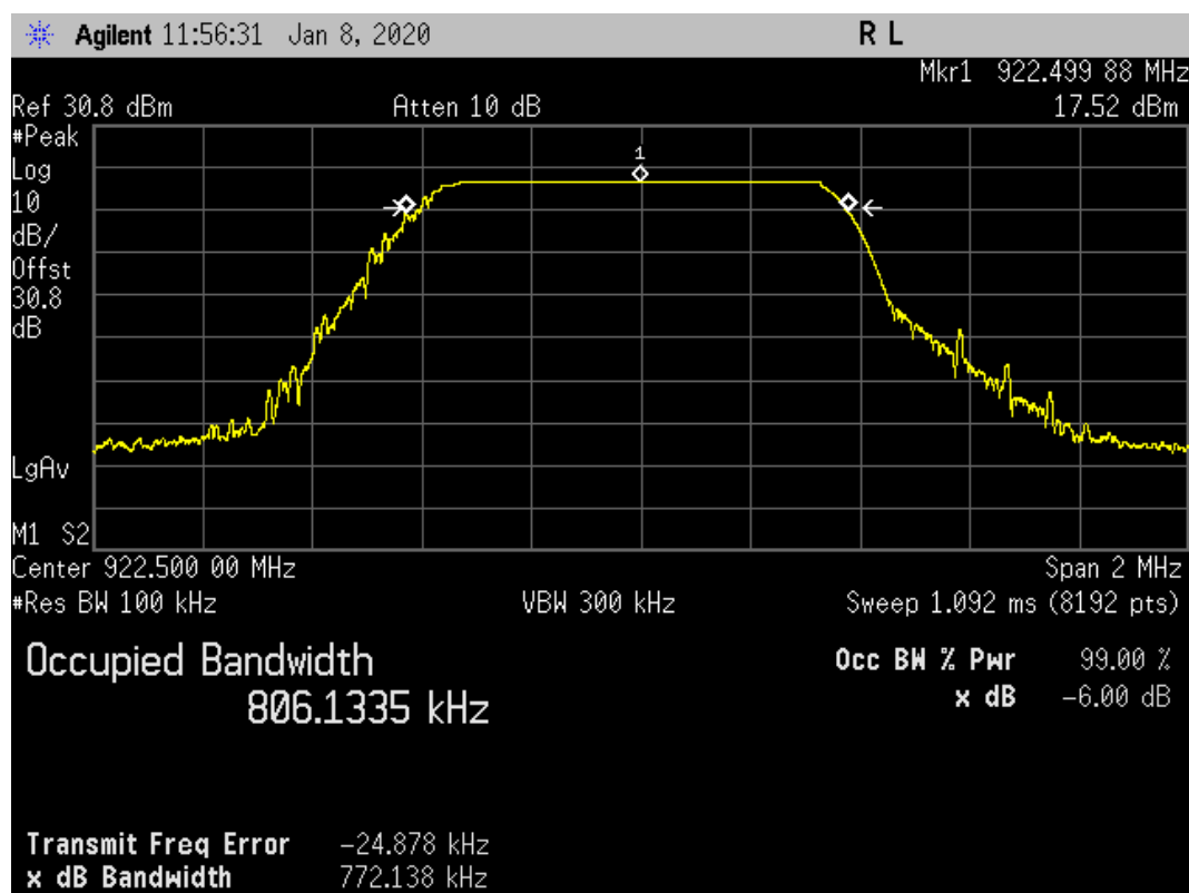
Plot for 6 dB Bandwidth (kHz) Nominal Temp & Volts
