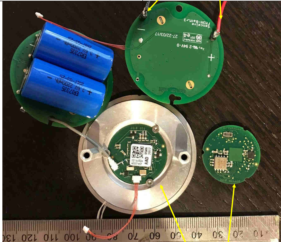
Antenna element PCB trace and feed point
