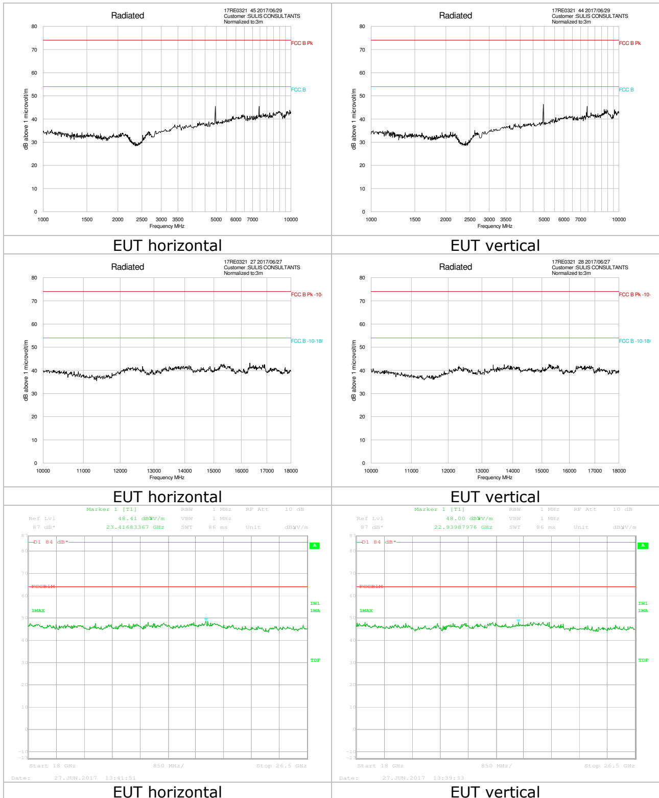
Figure 9: Radiated Spurious Emissions; Channel 25
