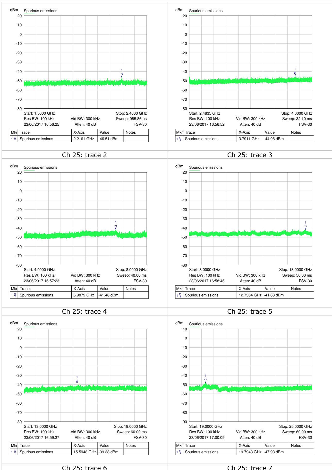
Figure 5: Emissions in non-restricted frequency bands
