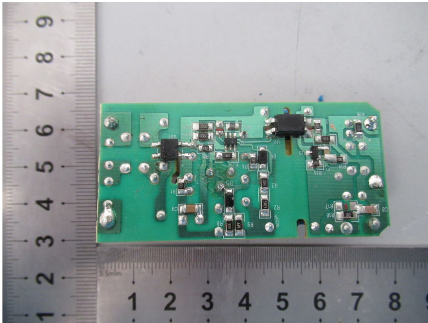
EUT – Modified Circuit Board View
