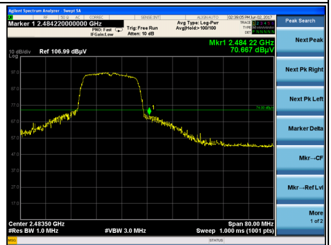
Band Edge, Left Side (Peak) - 802.11 n(20M) - CH 13
