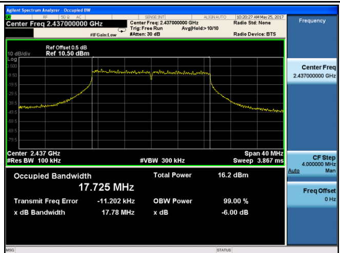
802.11n20 6dB Bandwidth - CH 6
