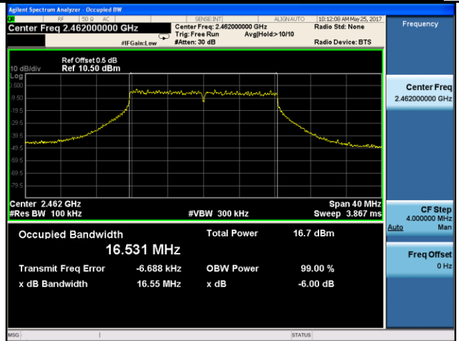
802.11g 6dB Bandwidth - CH 11
