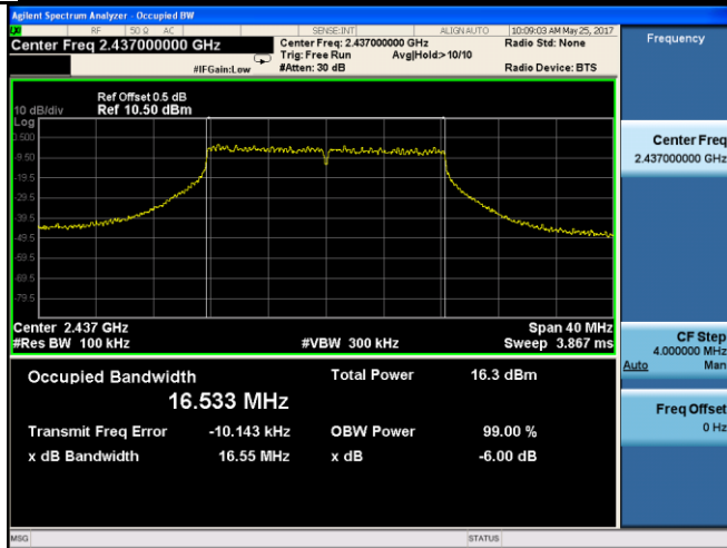
802.11g 6dB Bandwidth - CH 6
